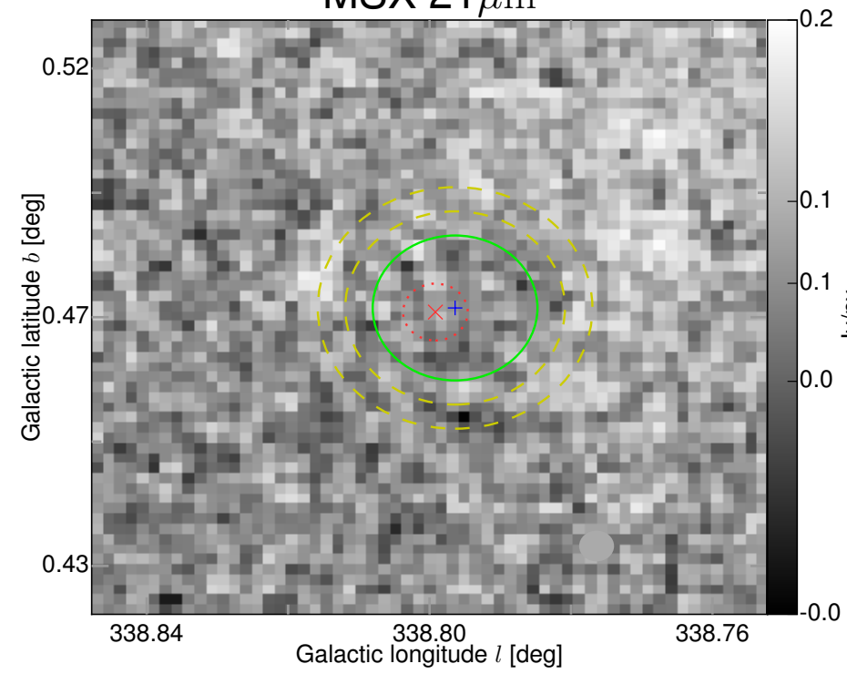
MSX 21 \mu\text{m}
