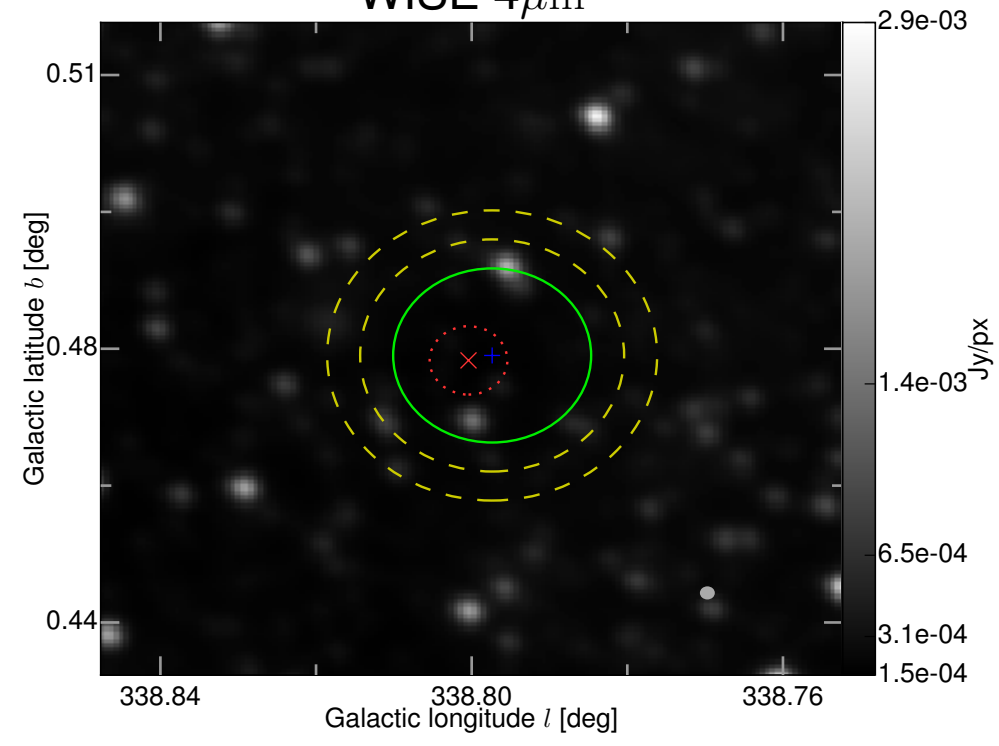
WISE 4 \mu\text{m}
