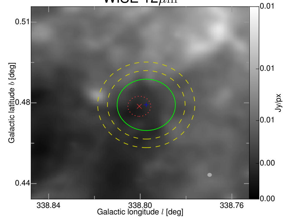
WISE 12 \mu\text{m}
