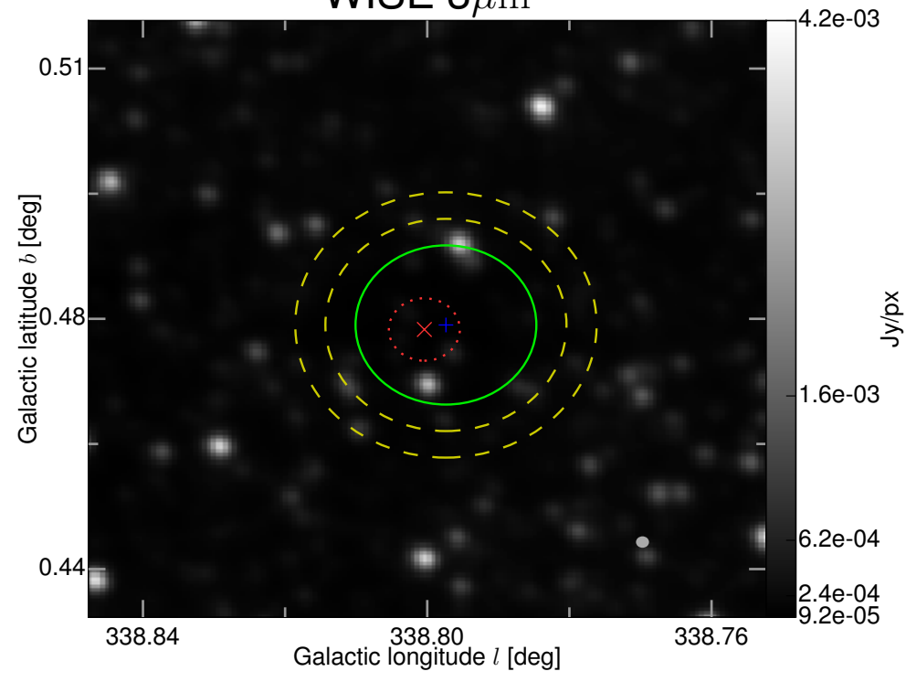
WISE 3 \mu\text{m}
