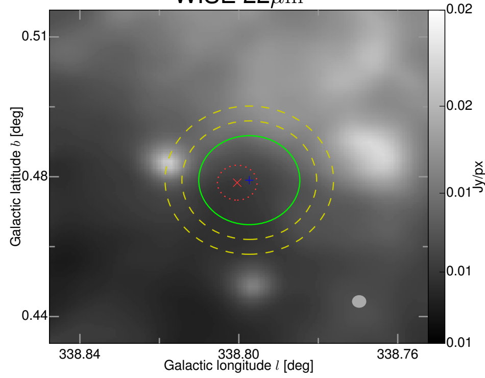
WISE 22 \mu\text{m}
