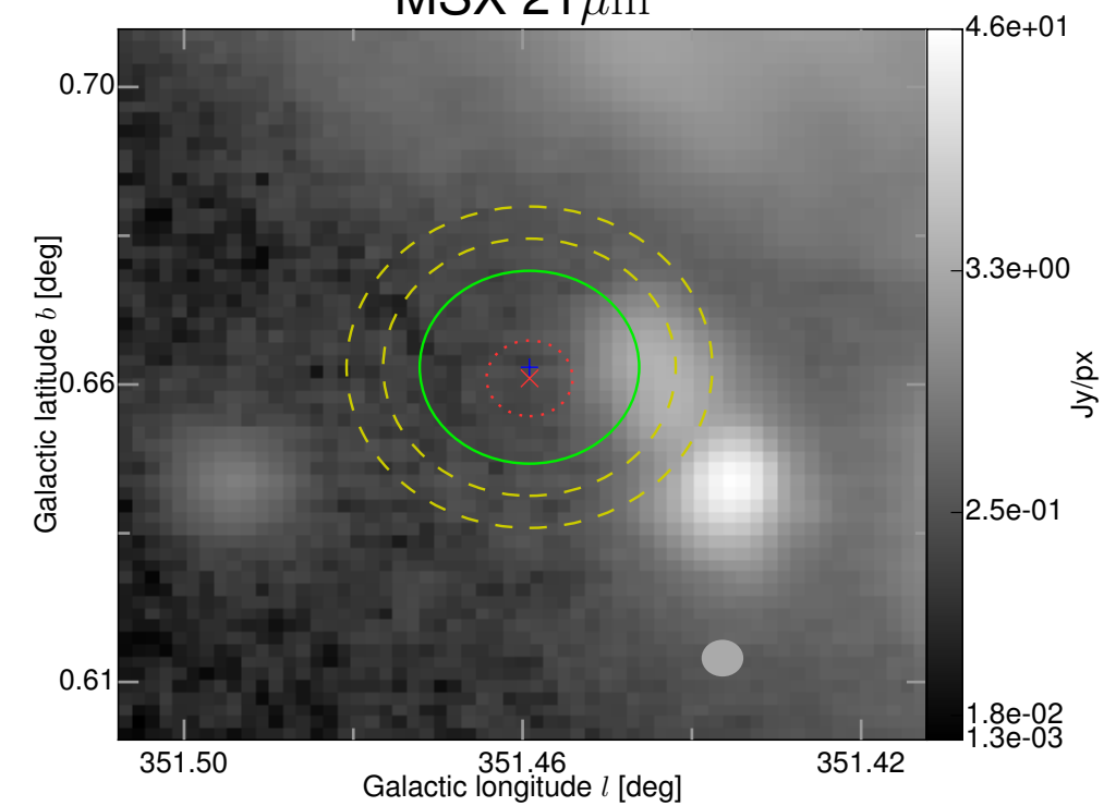
MSX 21\mu\text{m}
