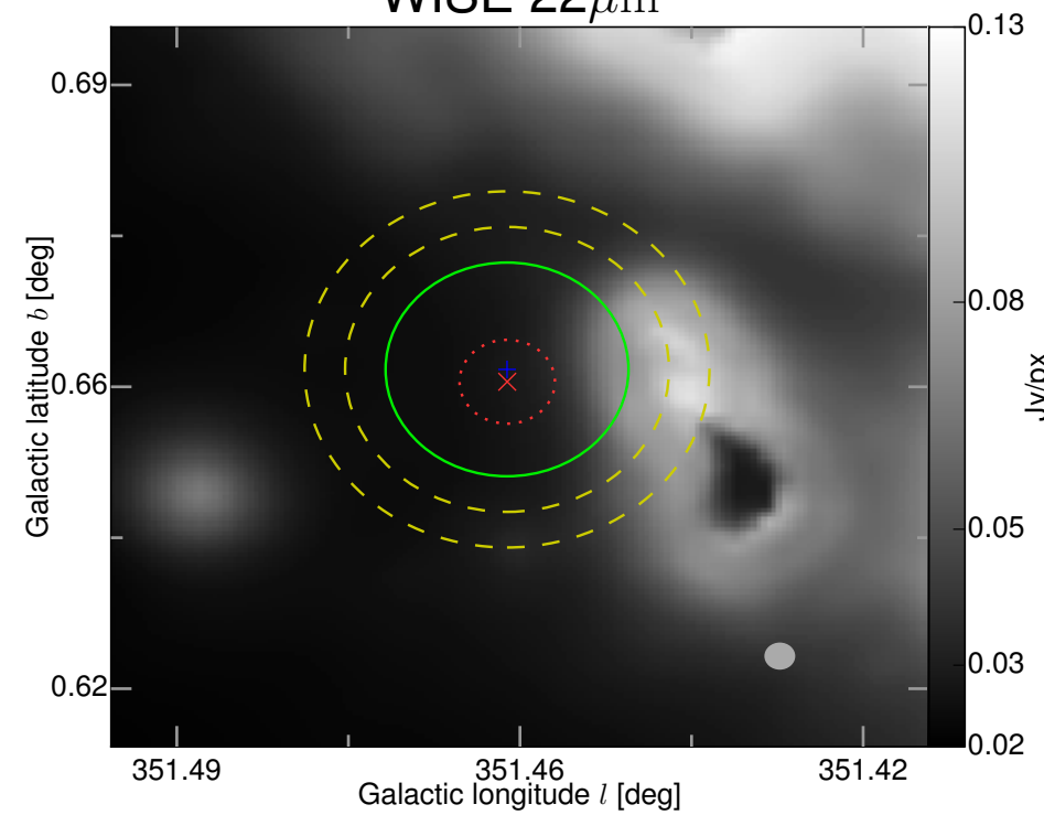
WISE 22\mu\text{m}
