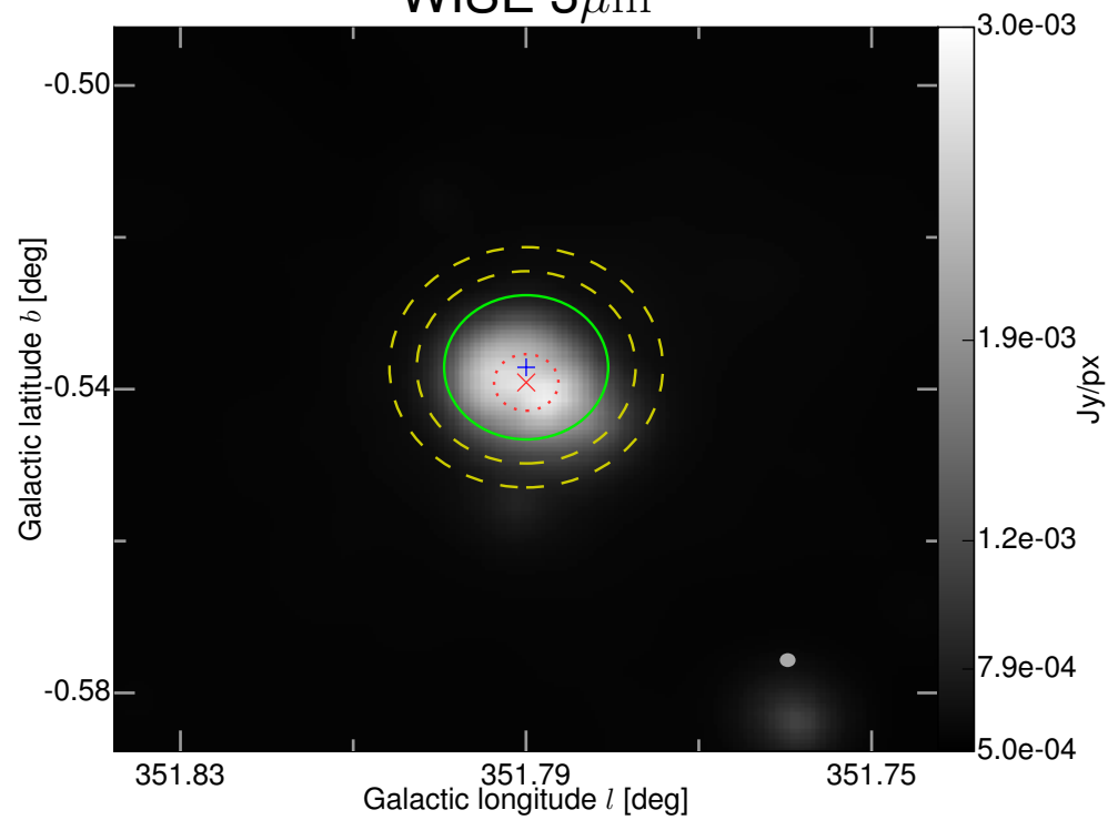
WISE 3 \mu\text{m}
