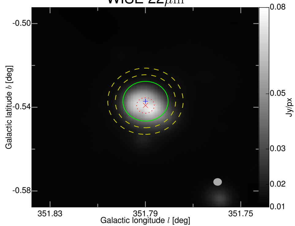
WISE 22 \mu\text{m}
