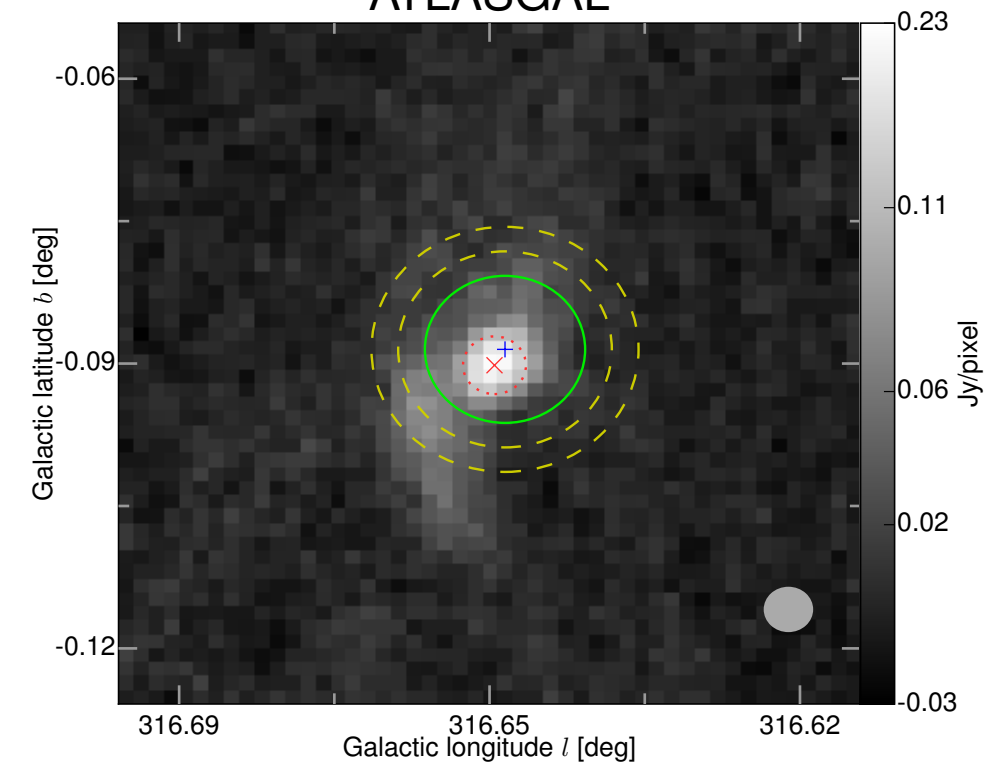
ATLASGAL
