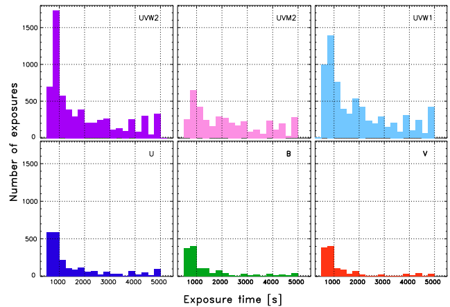
Figure 2. Exposure times of the XMM-OM images used to construct the XMM-SUSS, split by filter.
