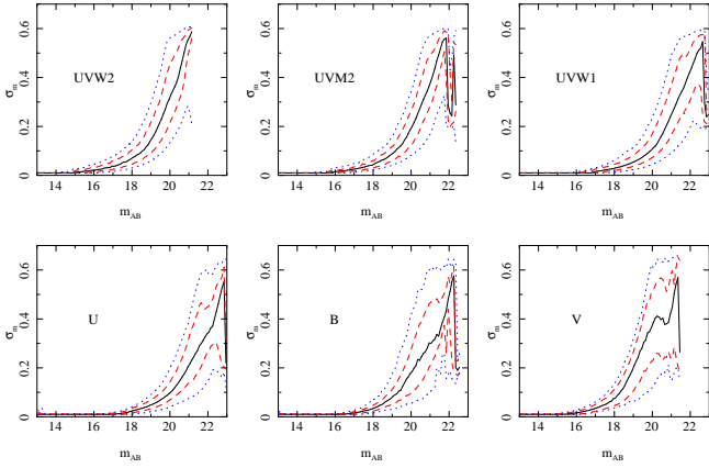
Figure 13. The distribution of magnitude uncertainties in the XMM-SUSS as a function of passband and magnitude. The solid black line shows the median error, the dashed red lines enclose 68 per cent of the distribution, and the blue dotted lines 95 per cent. The distributions were calculated in bins of 0.1 magnitude.
