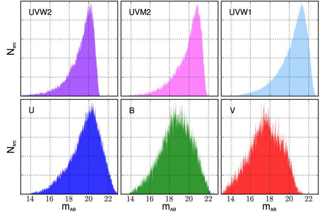
Figure 12. The normalized magnitude distributions of XMM-SUSS sources. Sources with quality flags are not included in the distributions. m_{\text{AB}} is the AB magnitude of sources and N_{\text{src}} the number of sources contained in each \Delta m_{\text{AB}} = 0.01 histogram bin.
