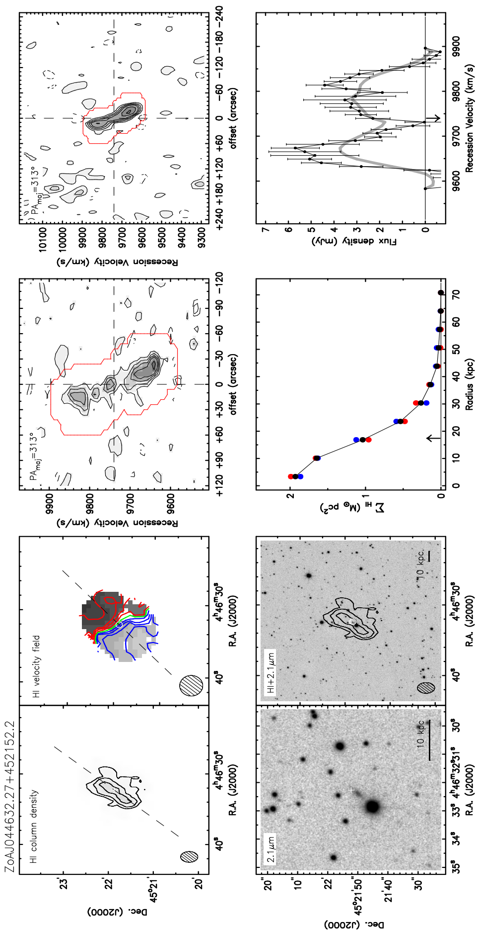
Figure A1. Resolved WSRT HI detections.
