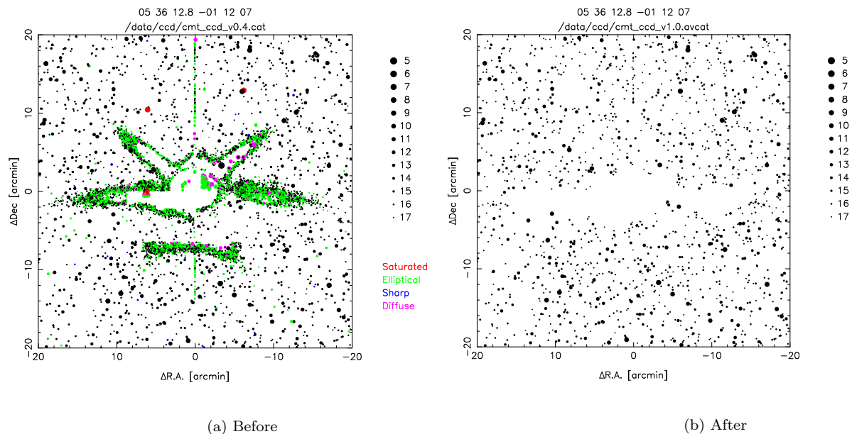
Figure 8: This figure shows the area around Epsilon Orionis (Alnilam) a 1.7 magnitude star, before and after the bright star mask has been applied.
