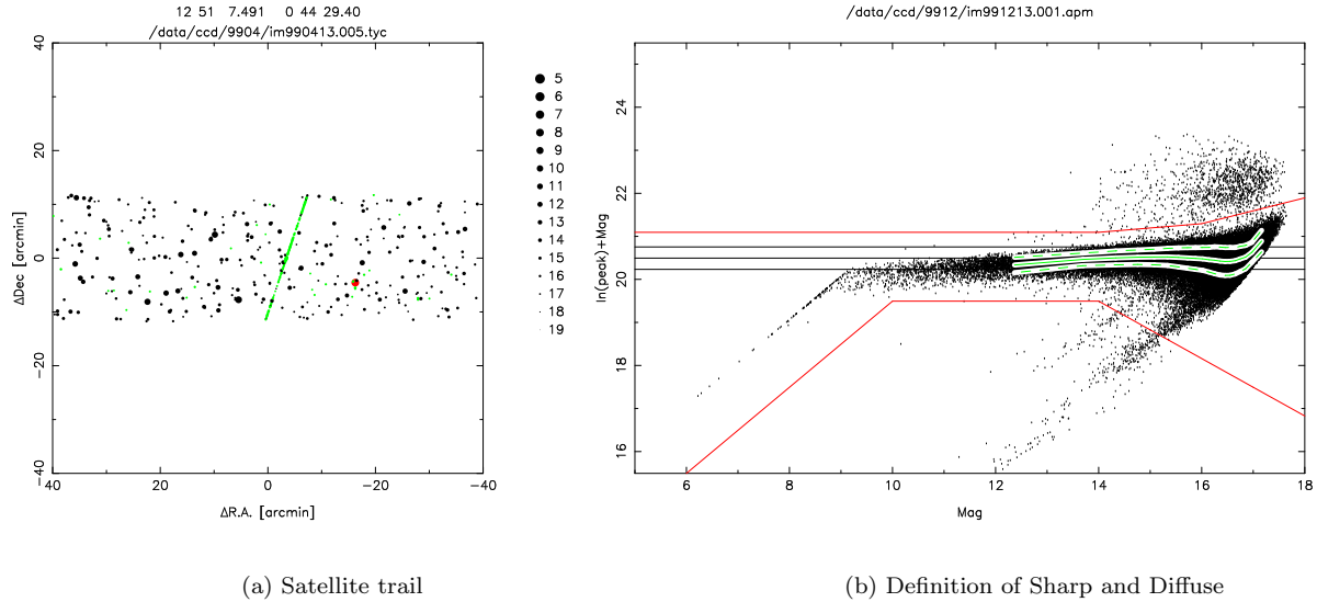
Figure 7: Plot (a) shows a satellite trail identified by the flagging of elliptical images (green). Plot (b) illustrates the definition of the Sharp and Diffuse flags. (\ln(\text{peak height}) + \text{magnitude}) is plotted against magnitude and the stellar locus identified. The red lines bound the acceptable images. The upper section images are then flagged as sharp and the lower section ones flagged as diffuse.
