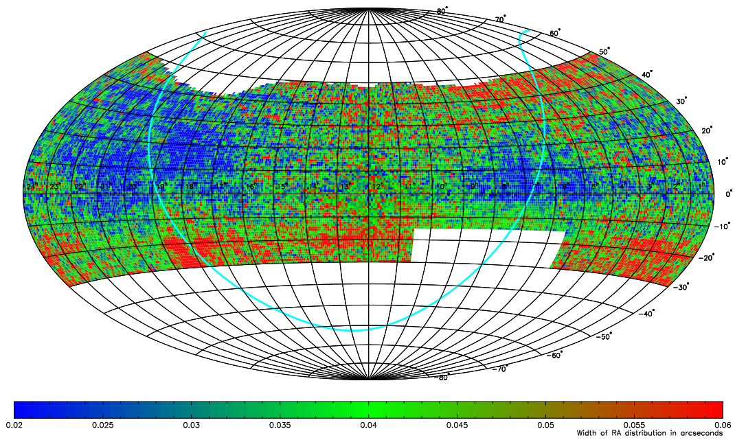
Figure 10: This shows the width of the RA difference distribution in a comparison between CMC14 and UCAC2. The Galactic plane is shown as the light blue line.
