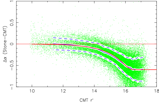
Figure 2: This plot shows the general trend in RA before correction caused by the CTE problem. This is a comparison, using observations taken during dark conditions, with respect to astrometric standards. A three-parameter model has been fitted to the data. This particular example comes from the beginning few months of the survey, which had problems with the camera controller. After this was replaced, the size of the effect reduced by a factor of 6. By the end of the survey, further modifications reduced the size of the effect by a further factor of 5 to 20 mas at r'_{\text{CMT}} = 17 . This is much smaller than the random errors at this magnitude.
