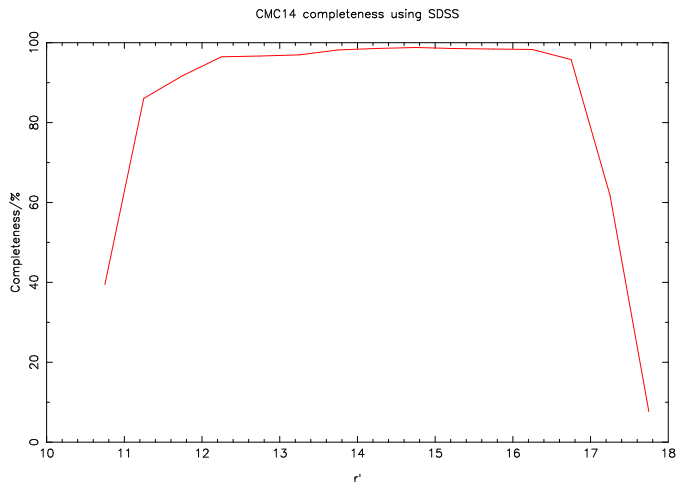
Figure 5: This shows the completeness of CMC14 by comparison with SDSS.
