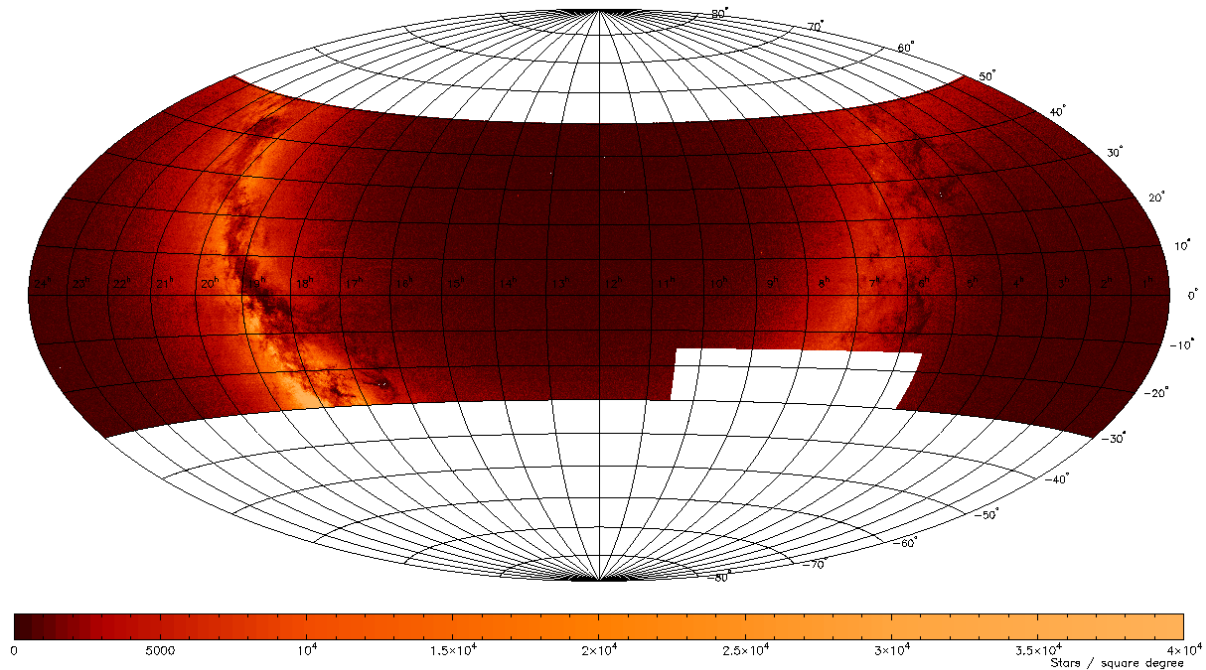
Figure 1: This shows the density of stars in CMC14.
