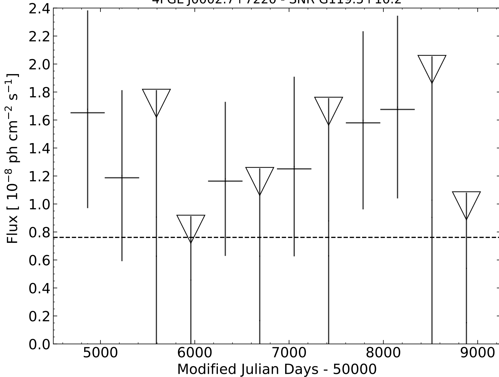
4FGL J0002.7+7220 - SNR G119.5+10.2
