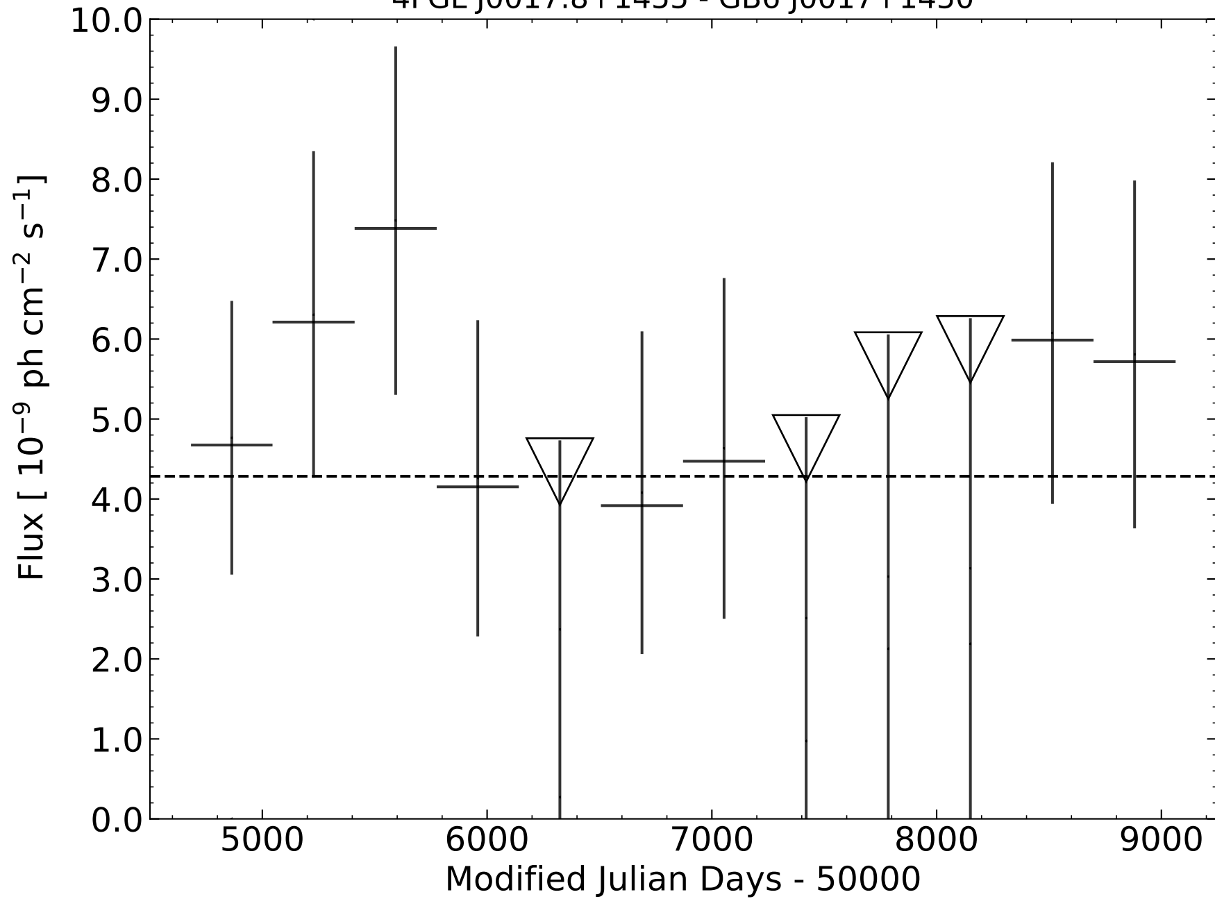
4FGL J0017.8+1455 - GB6 J0017+1450
