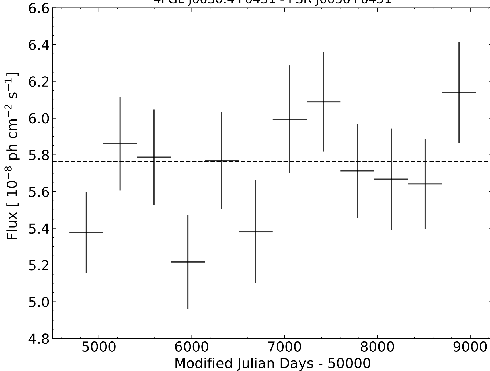
4FGL J0030.4+0451 - PSR J0030+0451
