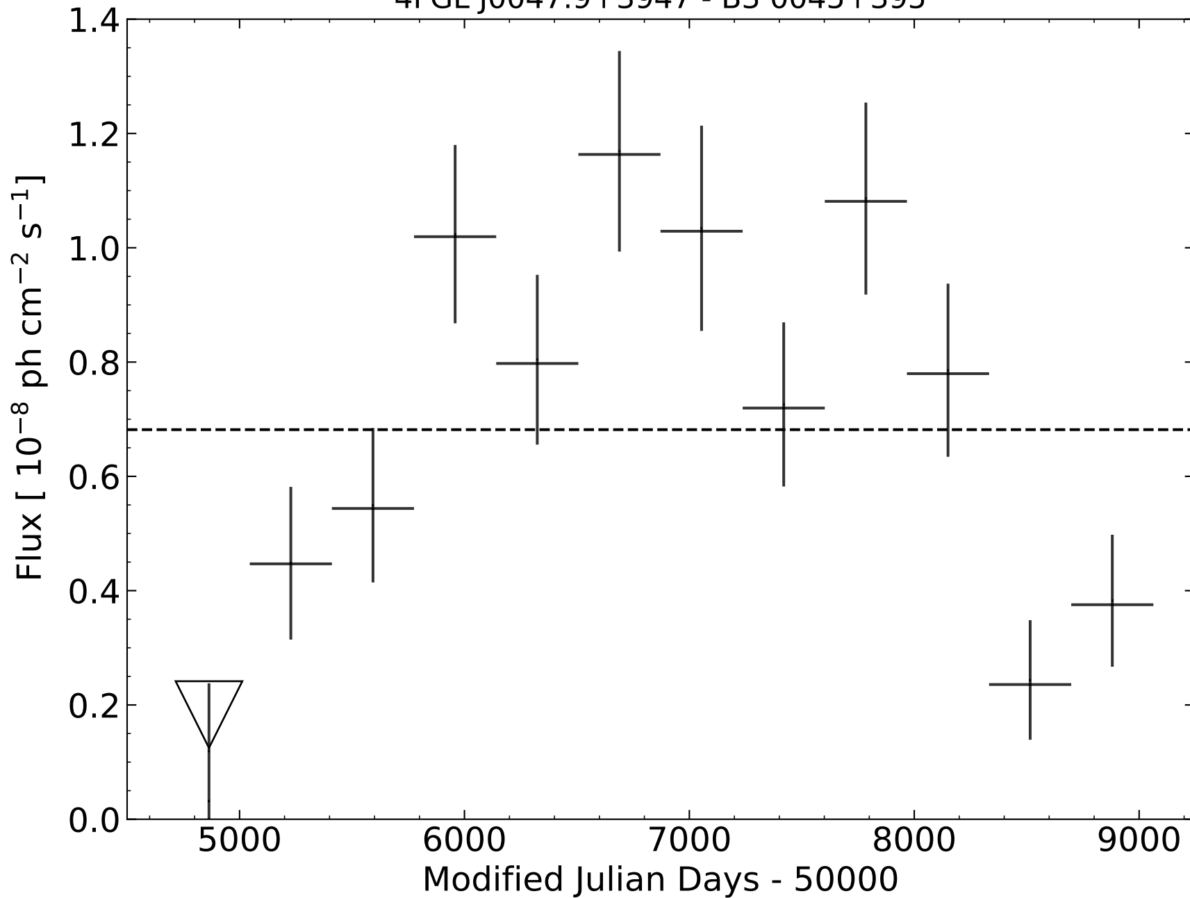
4FGL J0047.9+3947 - B3 0045+395
