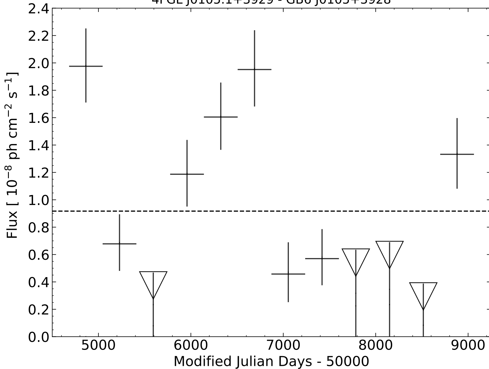
4FGL J0105.1+3929 - GB6 J0105+3928
