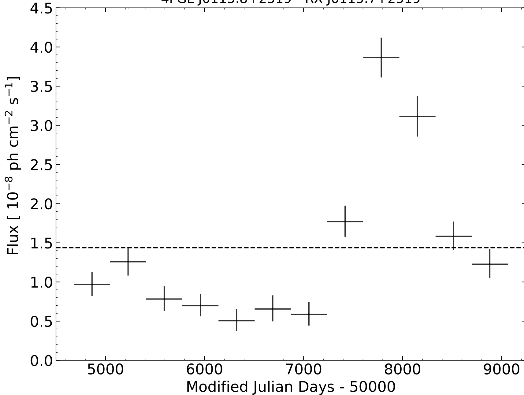
4FGL J0115.8+2519 - RX J0115.7+2519
