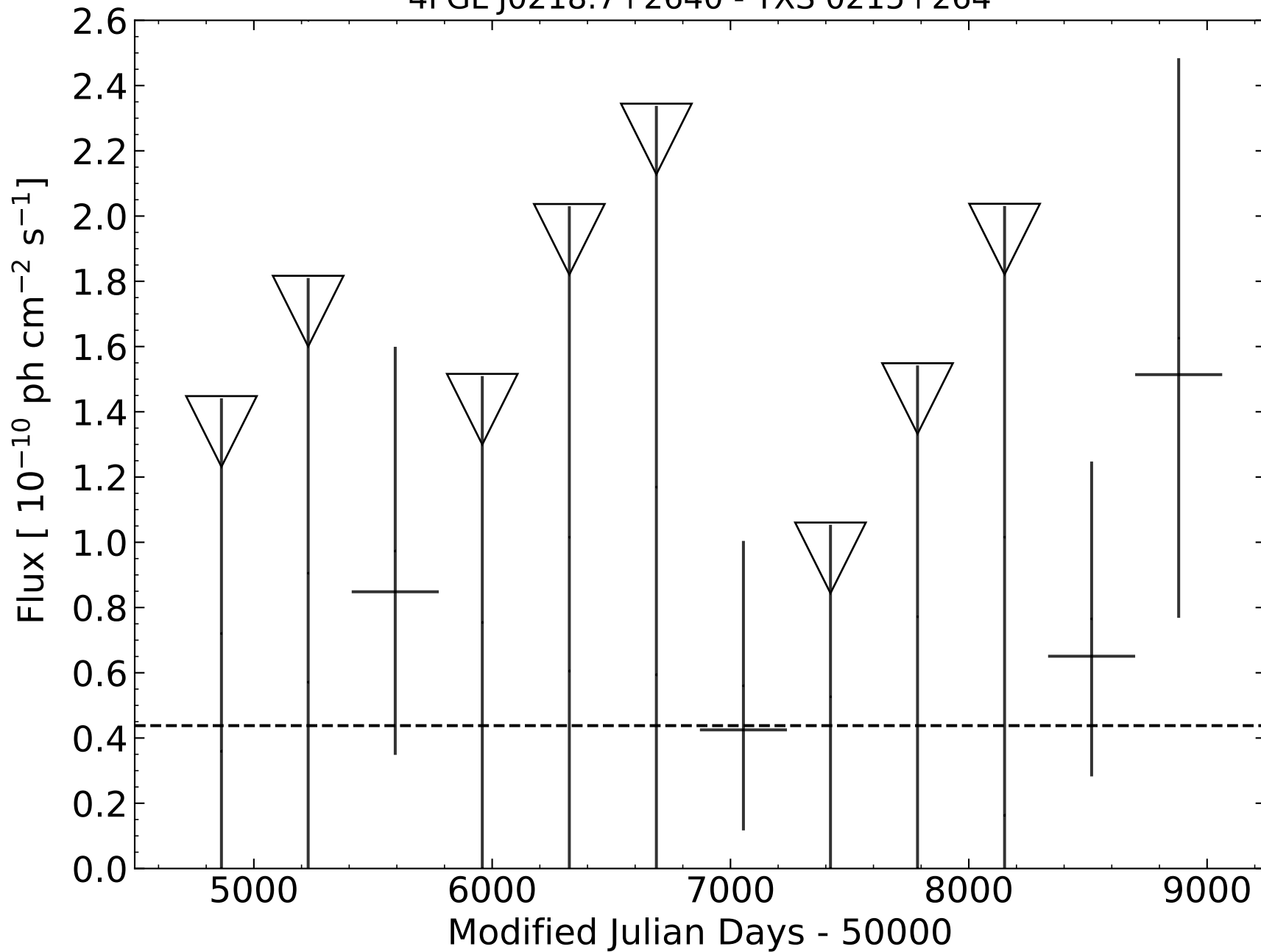
4FGL J0218.7+2640 - TXS 0215+264
