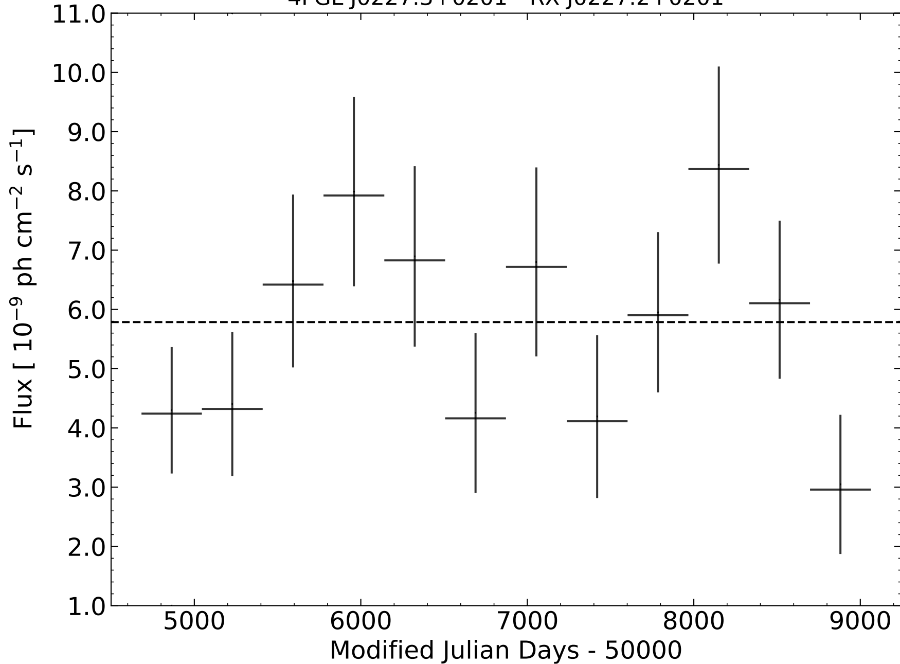
4FGL J0227.3+0201 - RX J0227.2+0201
