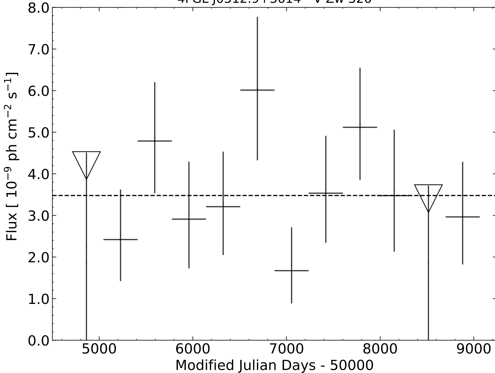
4FGL J0312.9+3614 - V Zw 326
