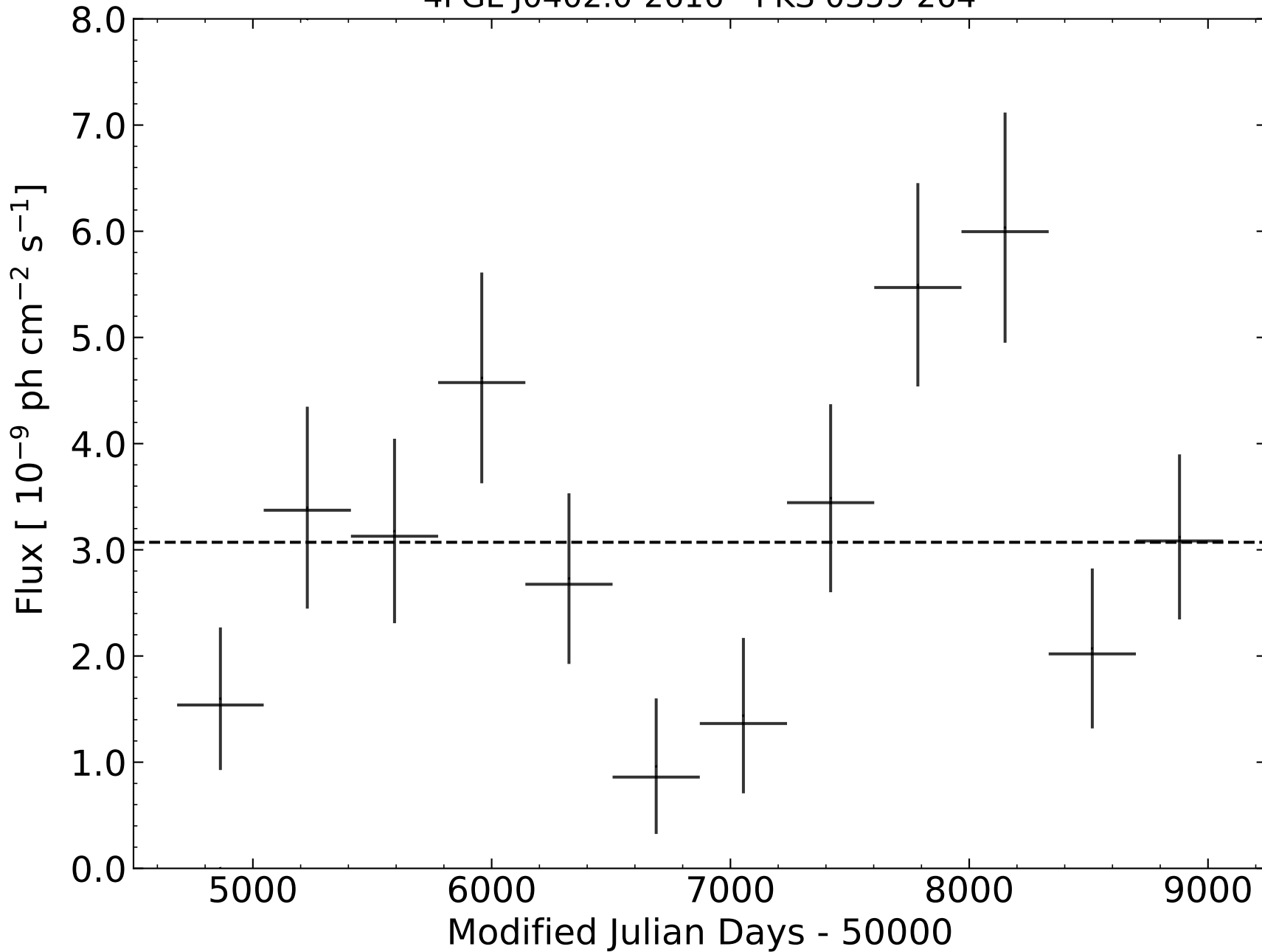
4FGL J0402.0-2616 - PKS 0359-264
