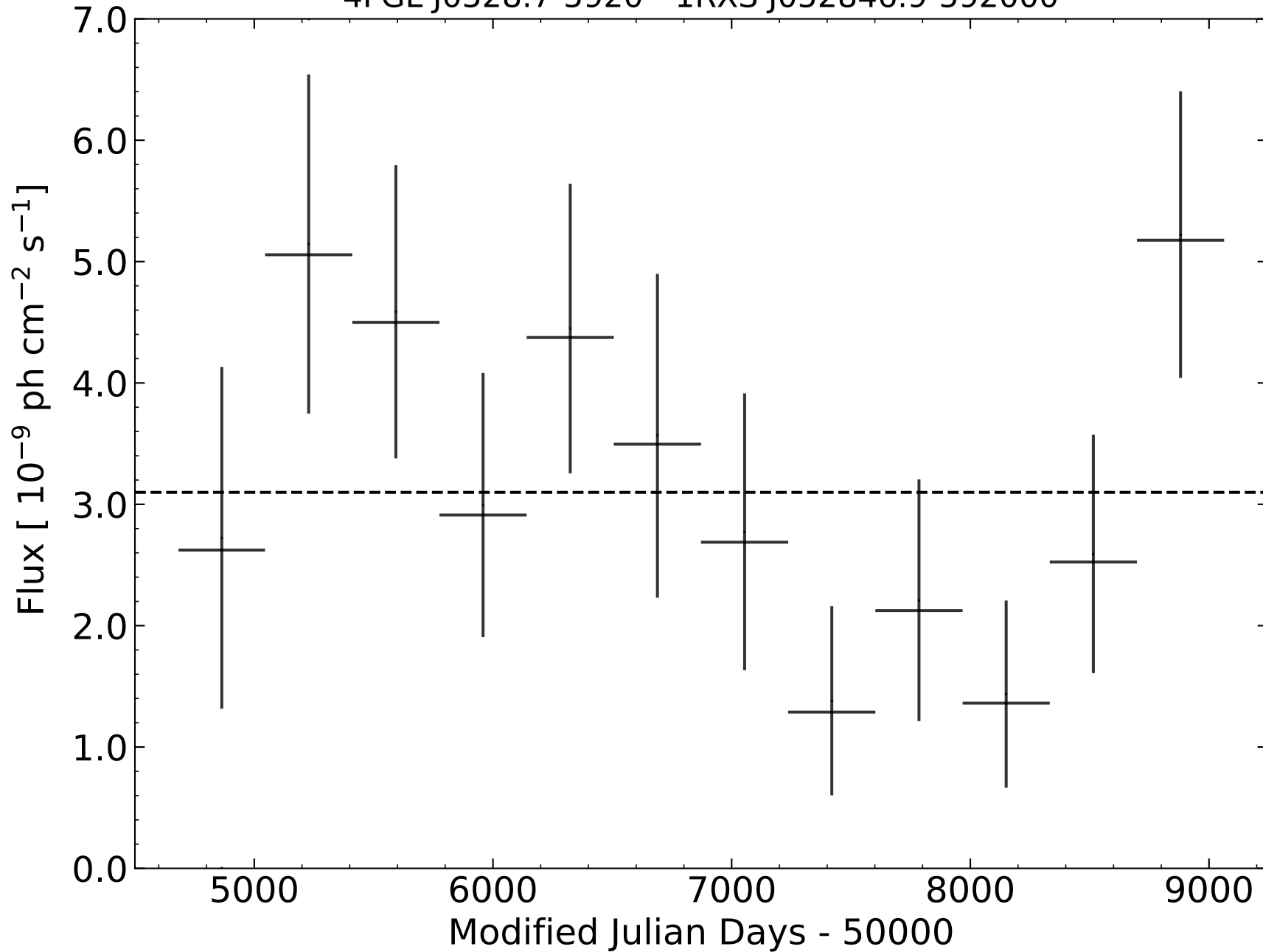
4FGL J0528.7-5920 - 1RXS J052846.9-592000
