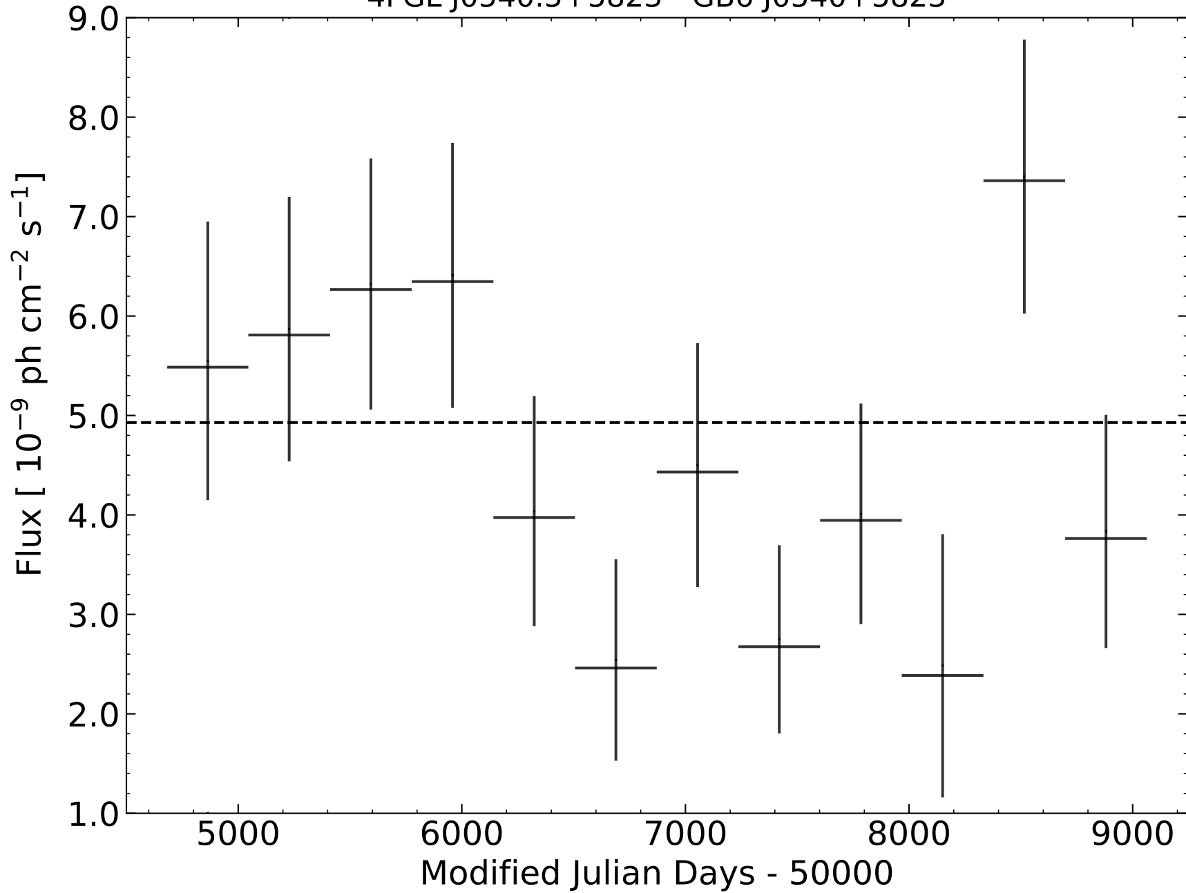
4FGL J0540.5+5823 - GB6 J0540+5823
