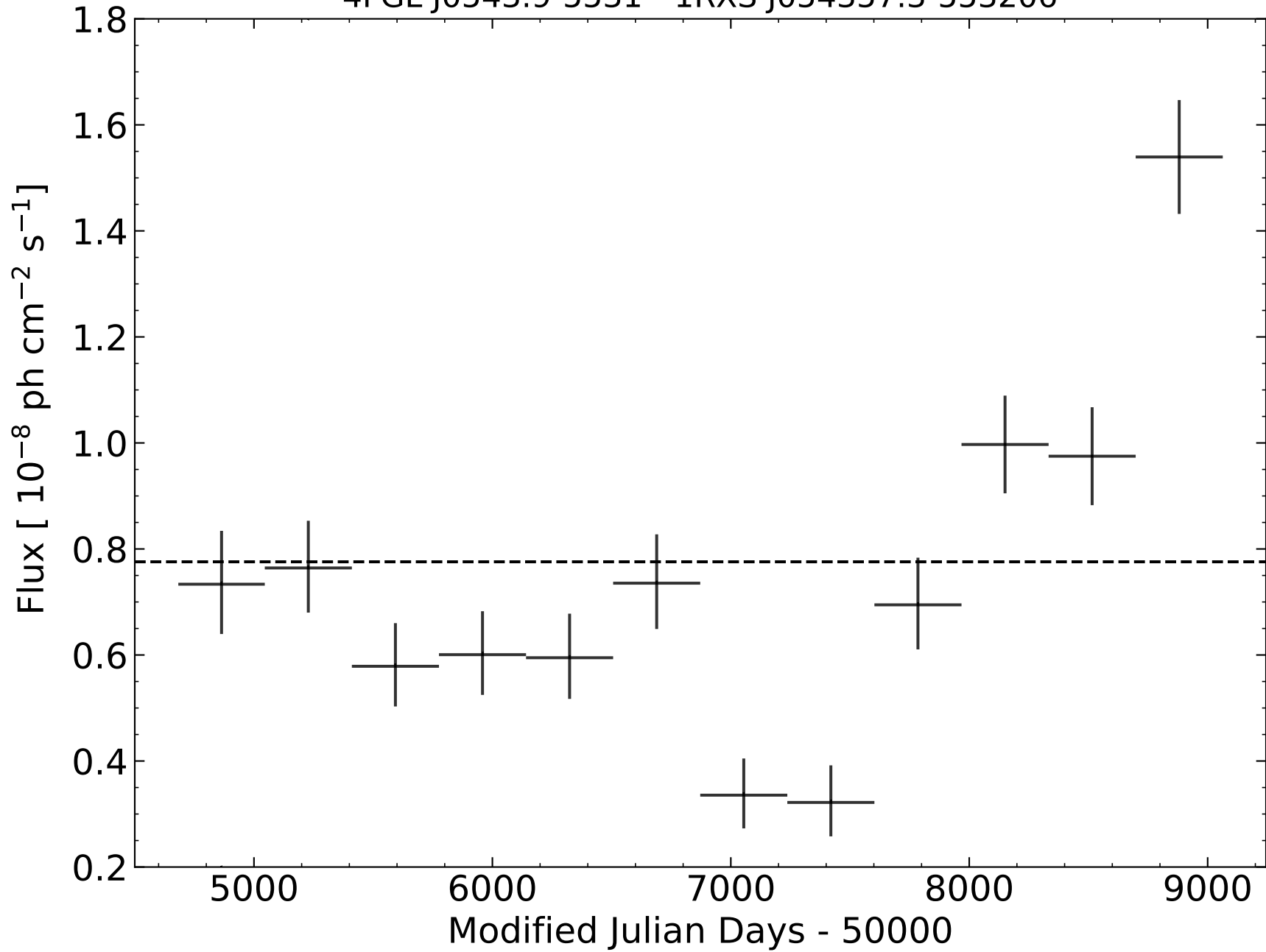
4FGL J0543.9-5531 - 1RXS J054357.3-553206
