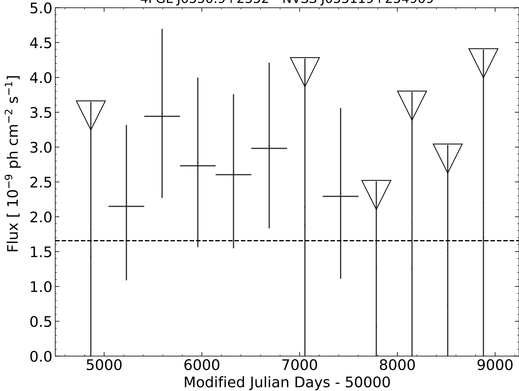
4FGL J0550.9+2552 - NVSS J055119+254909
