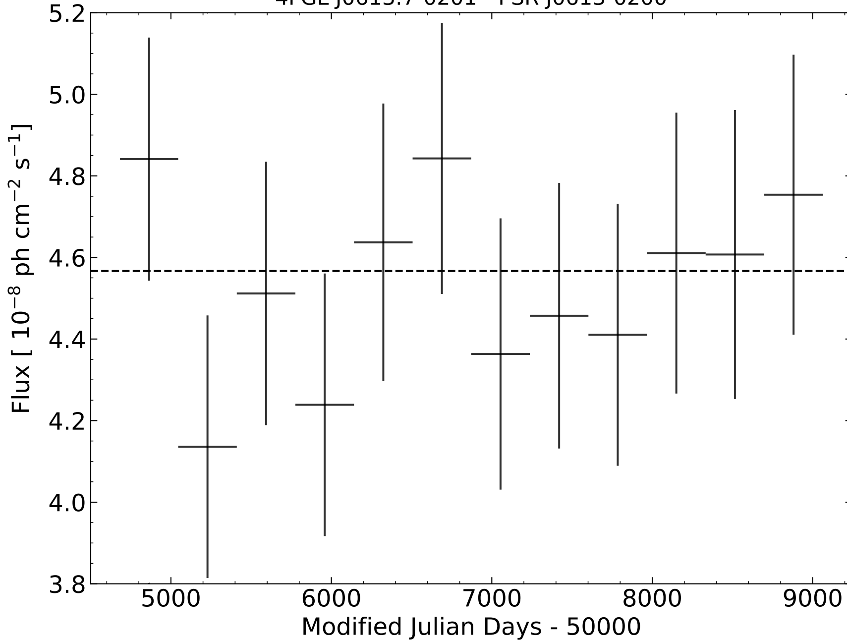
4FGL J0613.7-0201 - PSR J0613-0200
