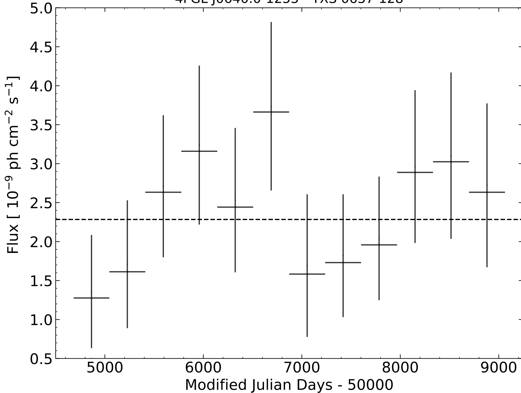
4FGL J0640.0-1253 - TXS 0637-128
