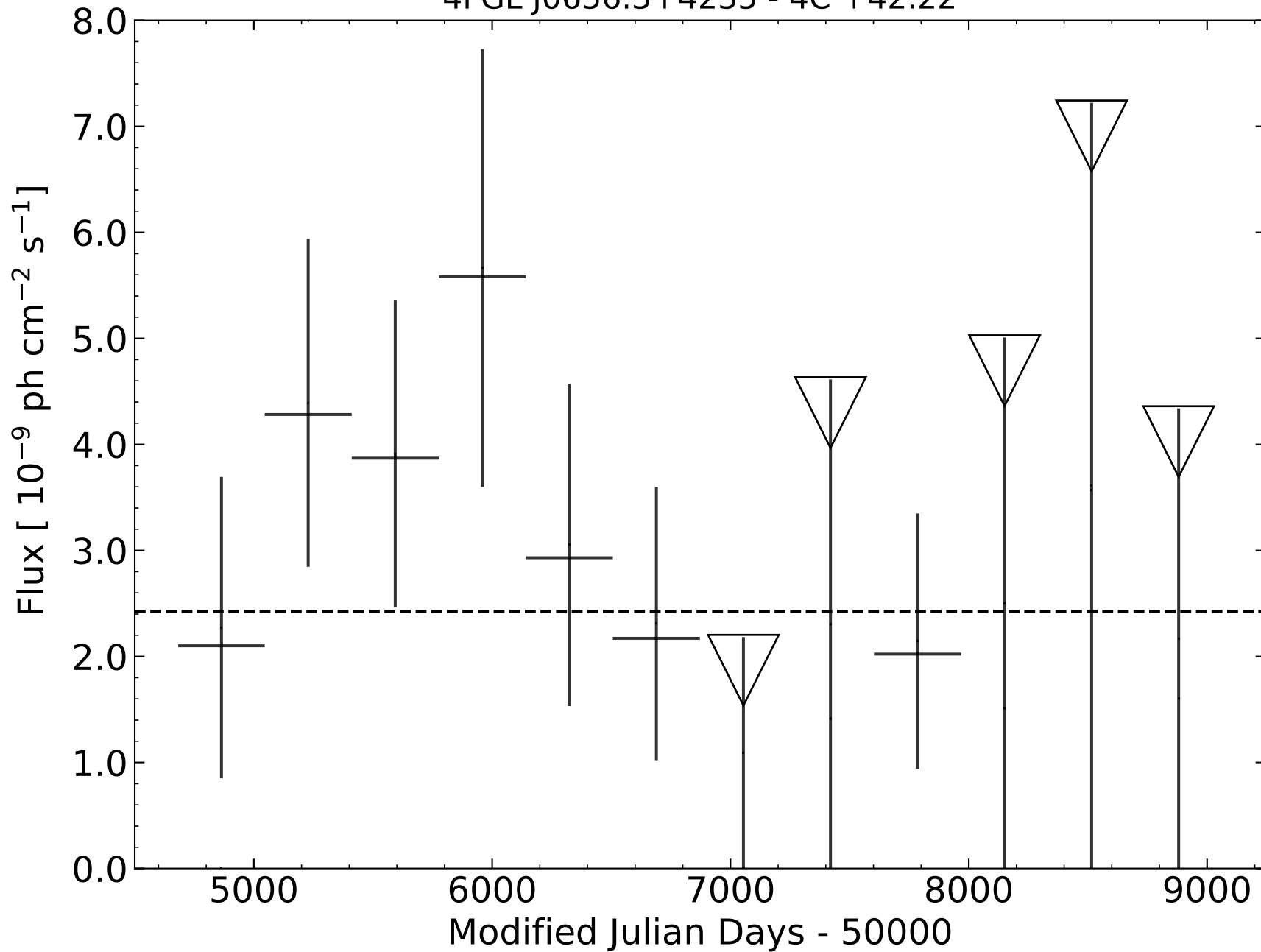
4FGL J0656.3+4235 - 4C +42.22
