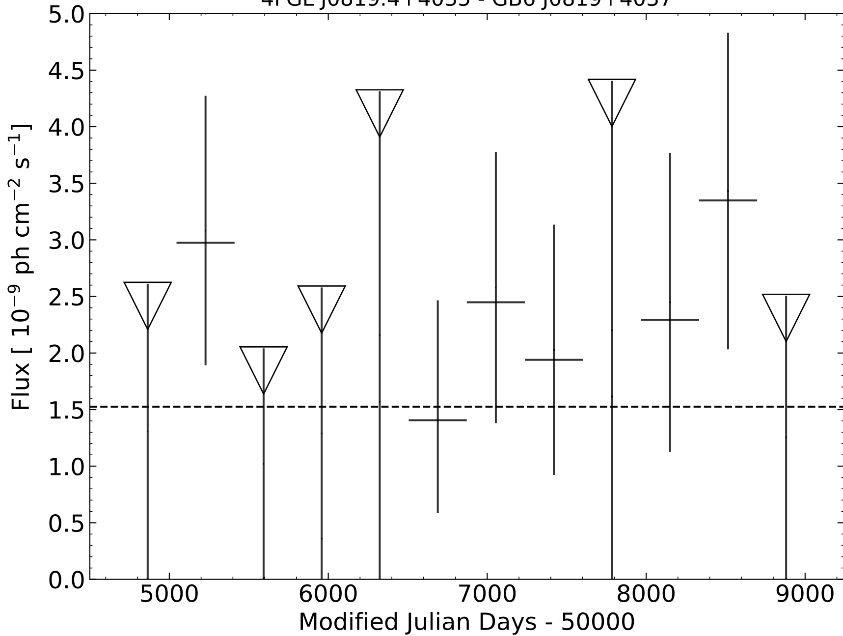
4FGL J0819.4+4035 - GB6 J0819+4037
