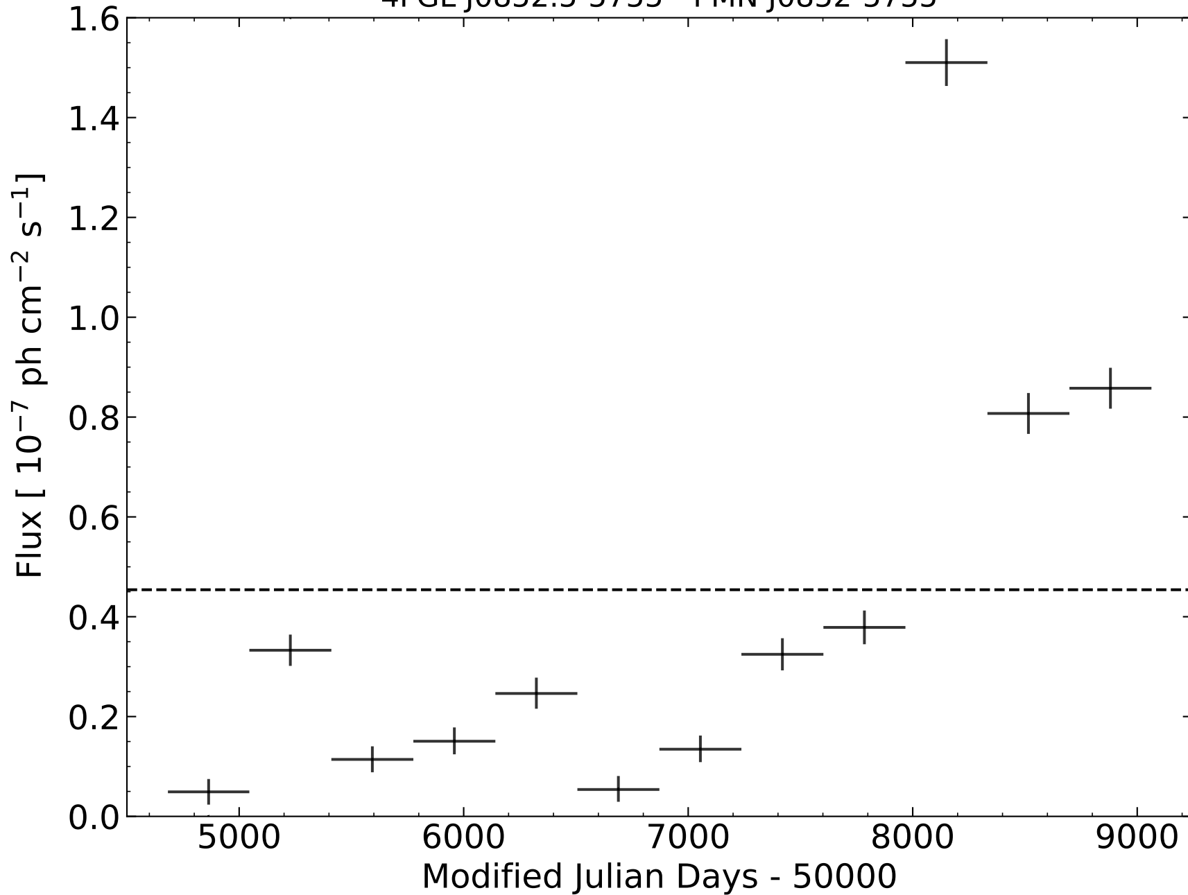
4FGL J0852.5-5755 - PMN J0852-5755
