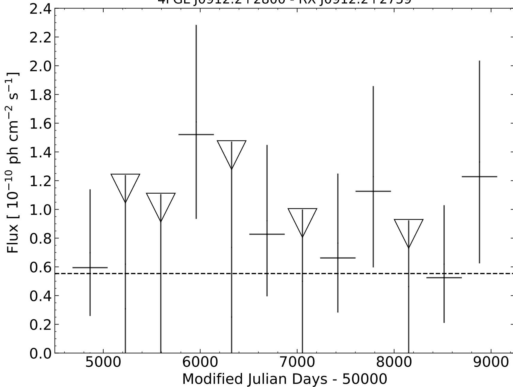
4FGL J0912.2+2800 - RX J0912.2+2759
