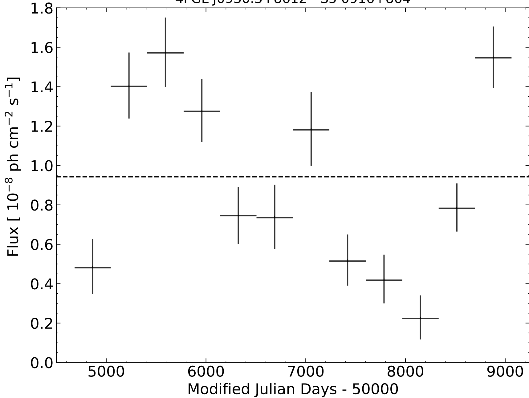
4FGL J0930.3+8612 - S5 0916+864
