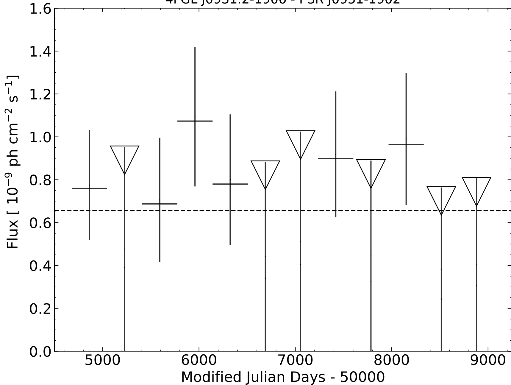
4FGL J0931.2-1906 - PSR J0931-1902
