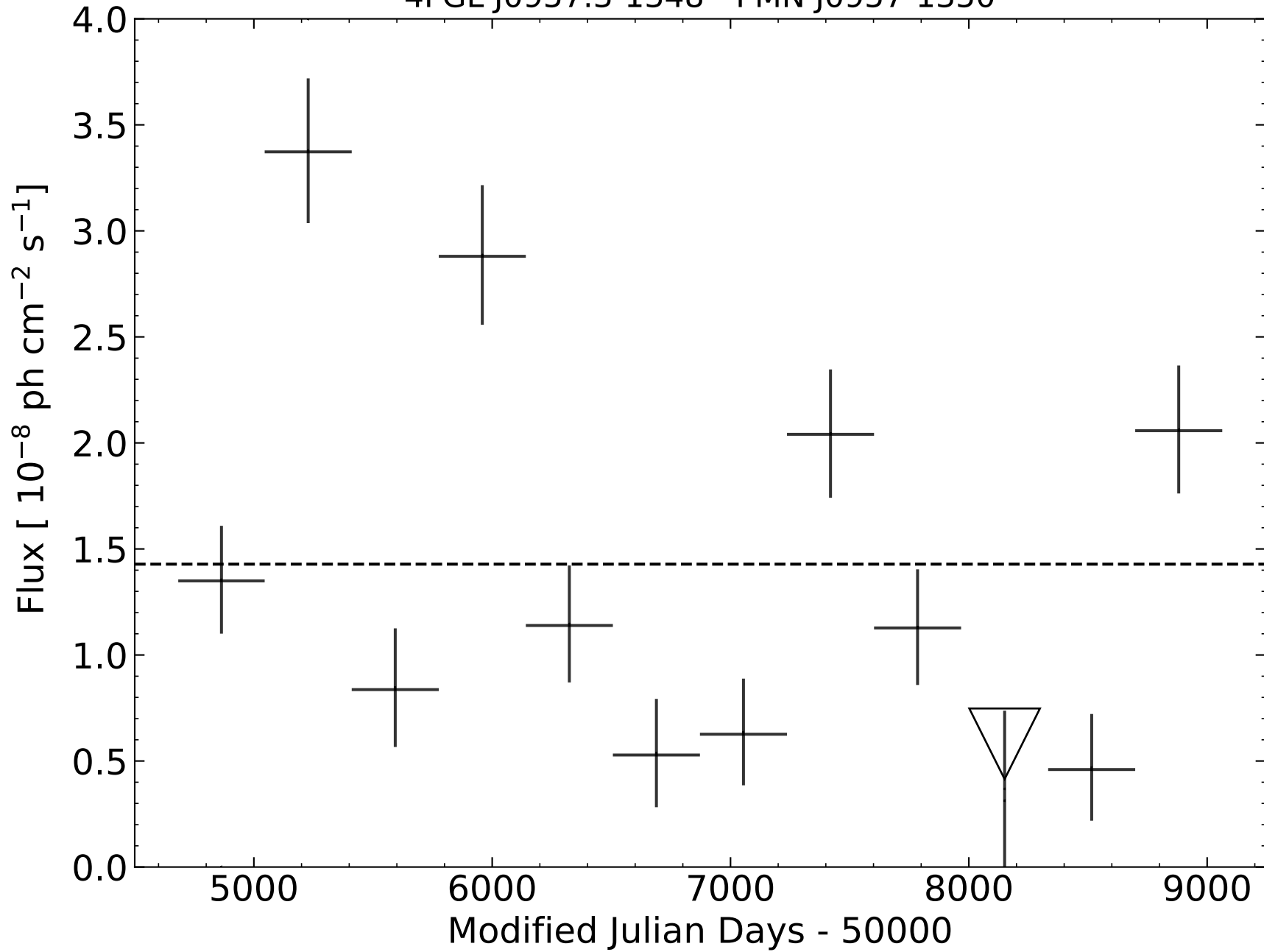
4FGL J0957.3-1348 - PMN J0957-1350
