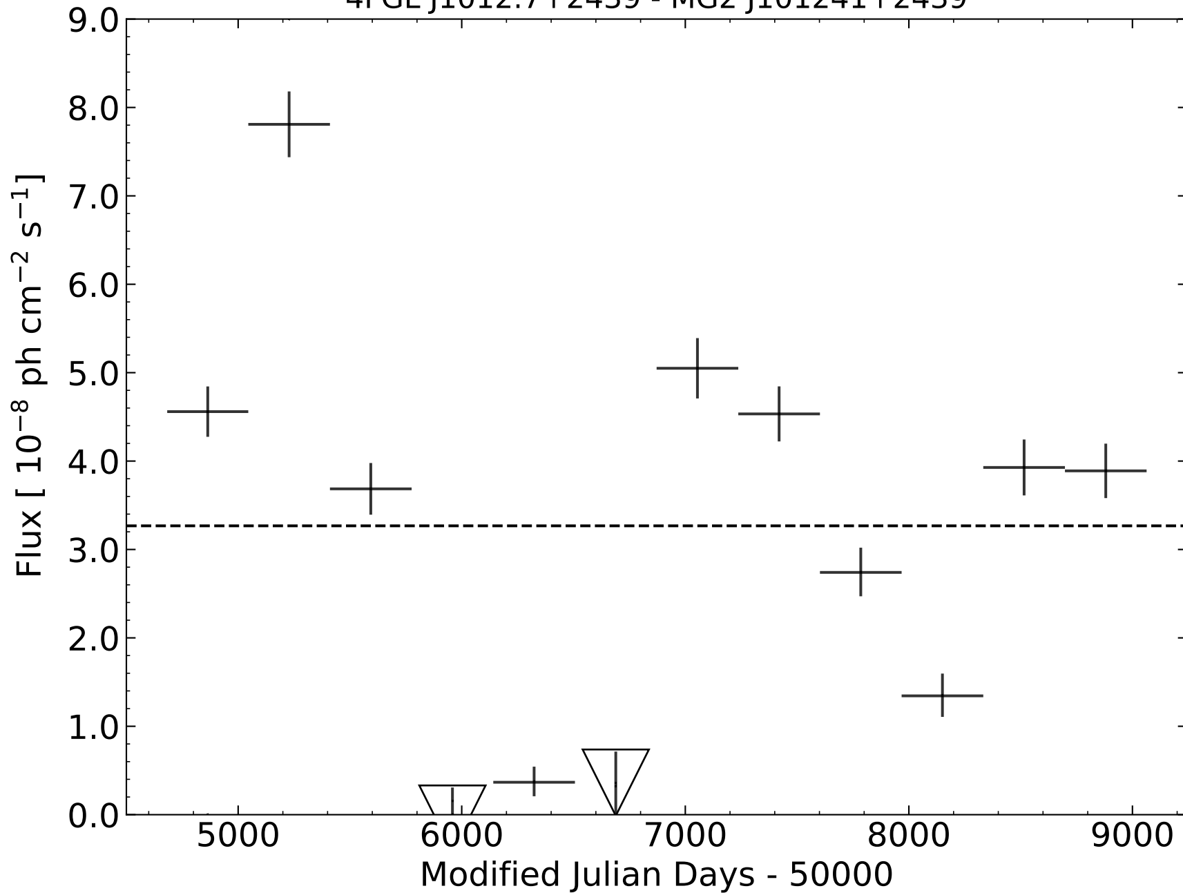
4FGL J1012.7+2439 - MG2 J101241+2439
