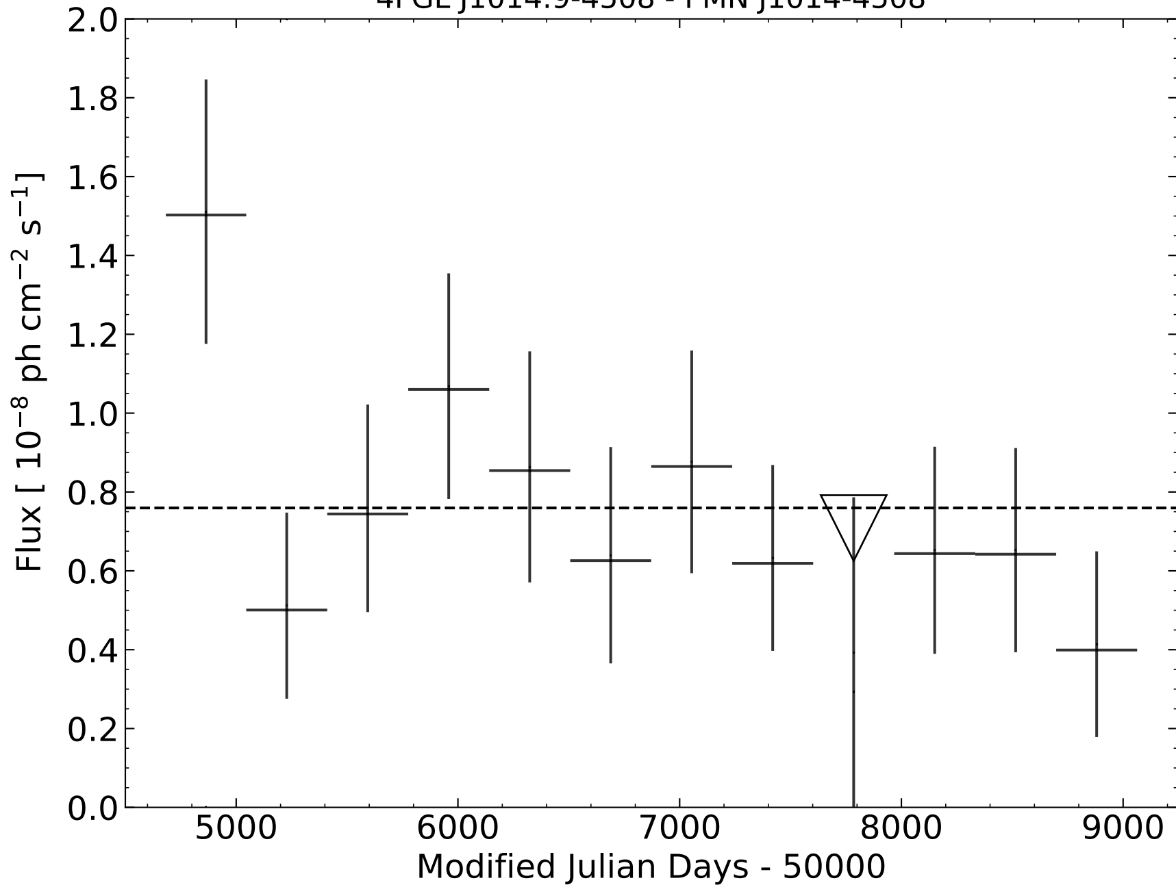
4FGL J1014.9-4508 - PMN J1014-4508
