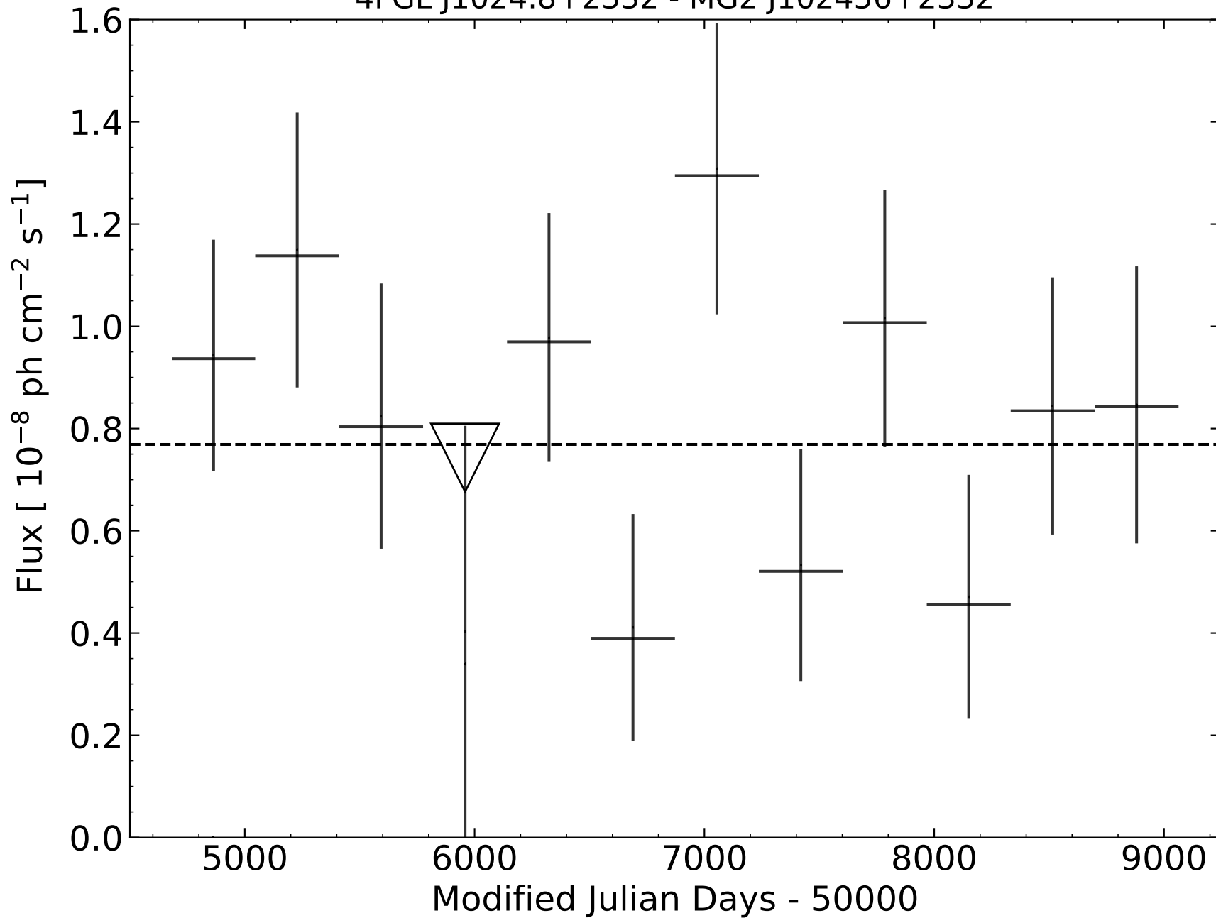
4FGL J1024.8+2332 - MG2 J102456+2332
