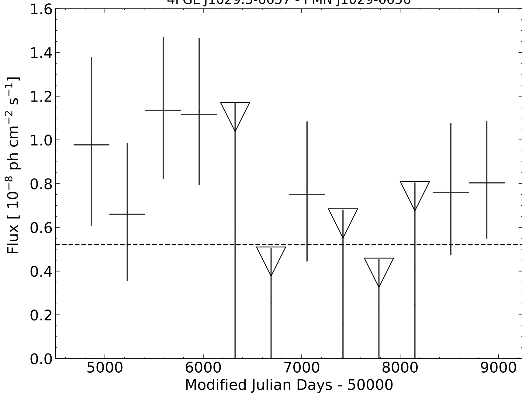
4FGL J1029.3-6657 - PMN J1029-6656
