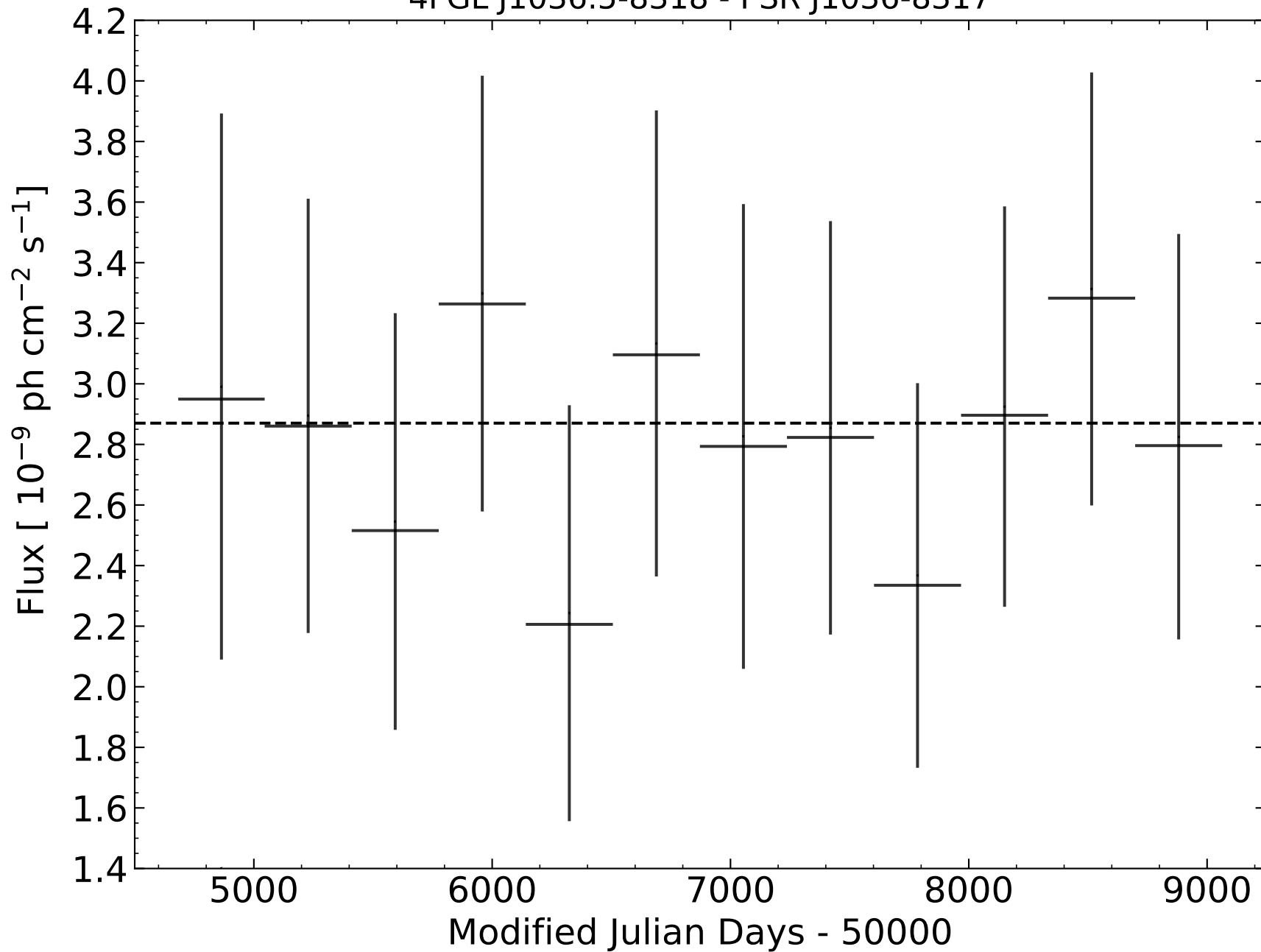
4FGL J1036.5-8318 - PSR J1036-8317
