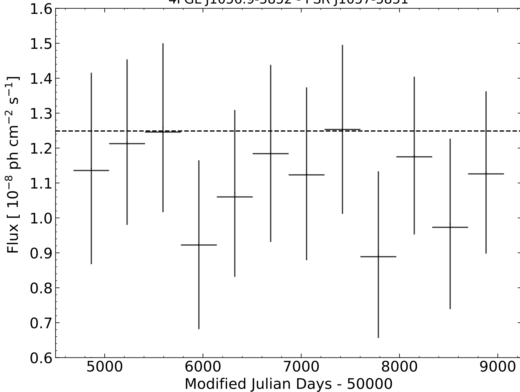
4FGL J1056.9-5852 - PSR J1057-5851
