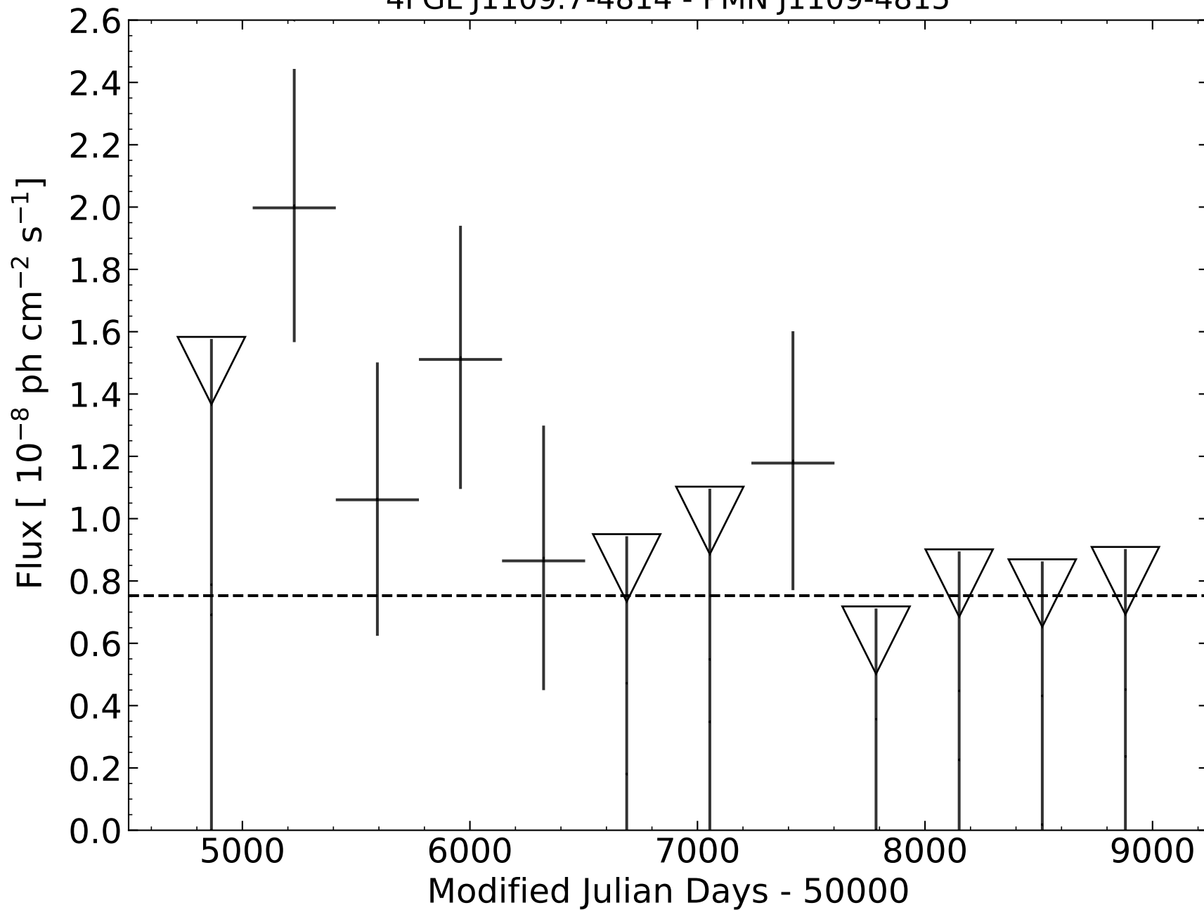
4FGL J1109.7-4814 - PMN J1109-4815
