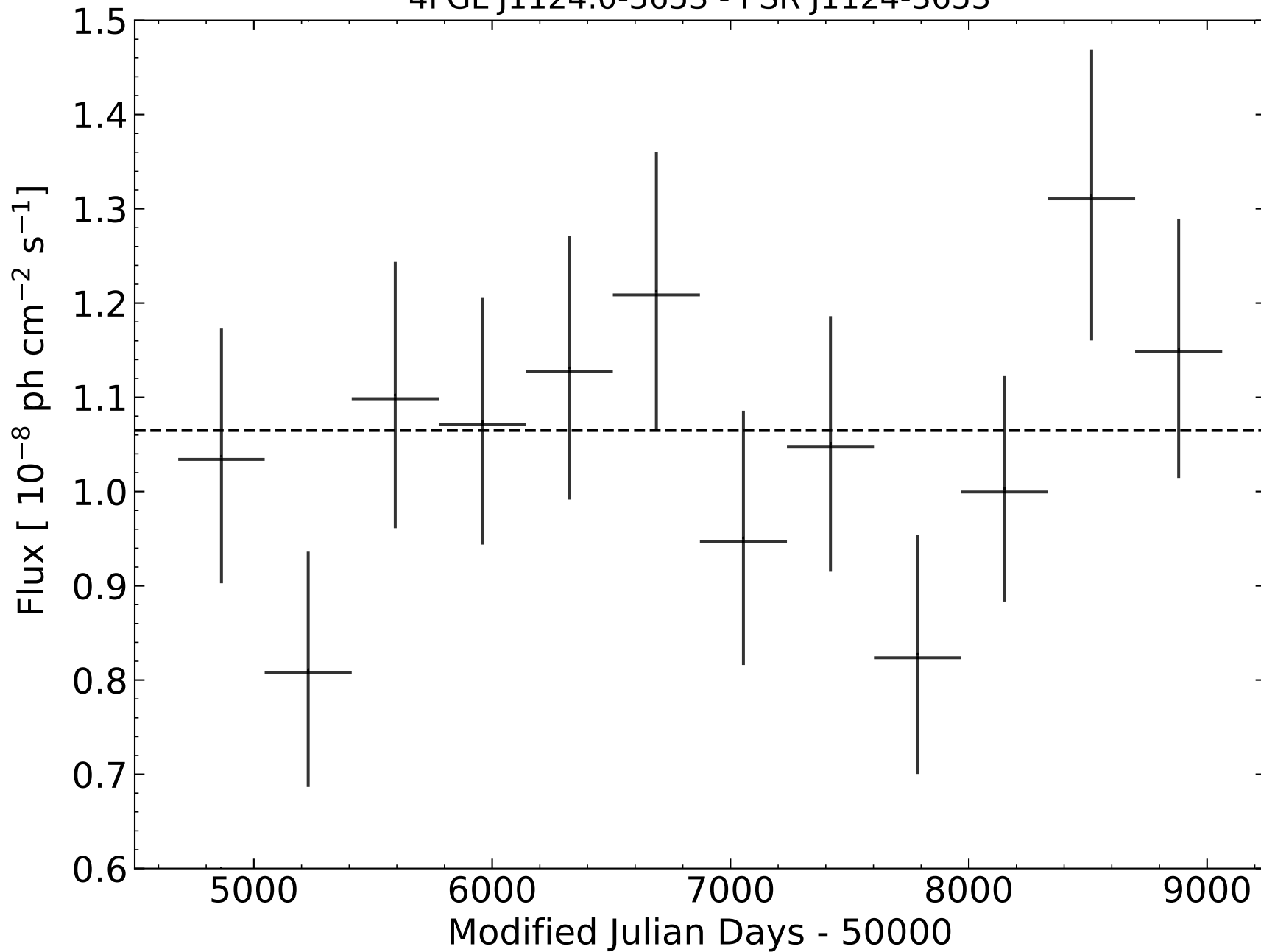
4FGL J1124.0-3653 - PSR J1124-3653
