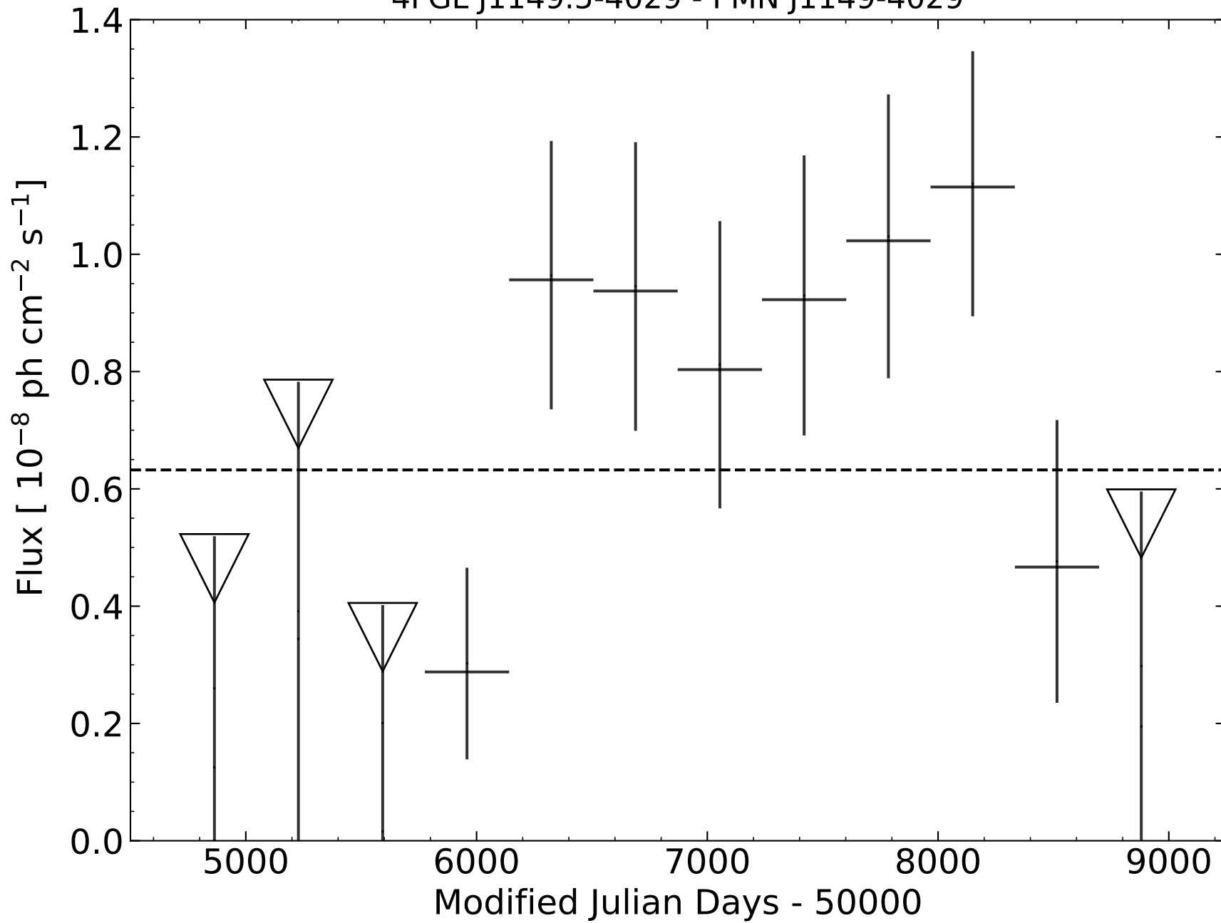
4FGL J1149.5-4029 - PMN J1149-4029
