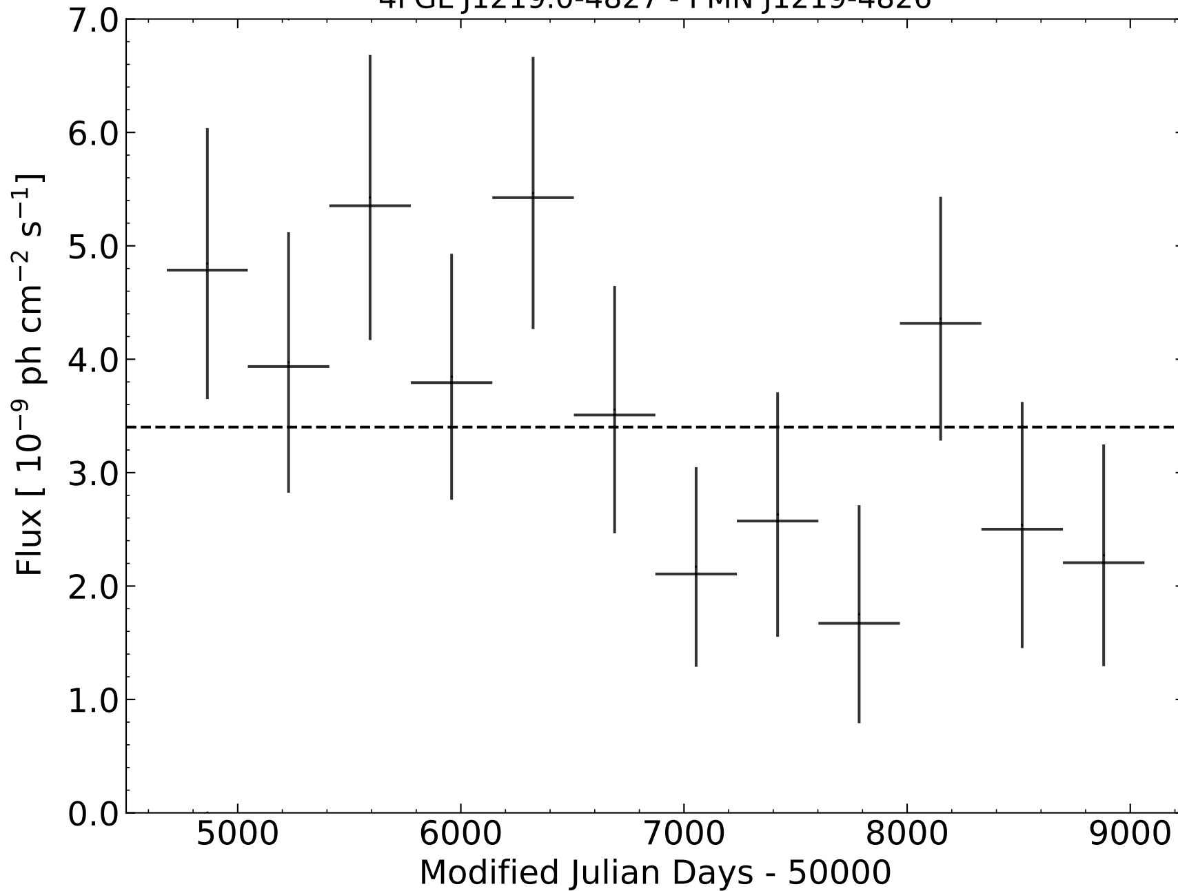
4FGL J1219.0-4827 - PMN J1219-4826
