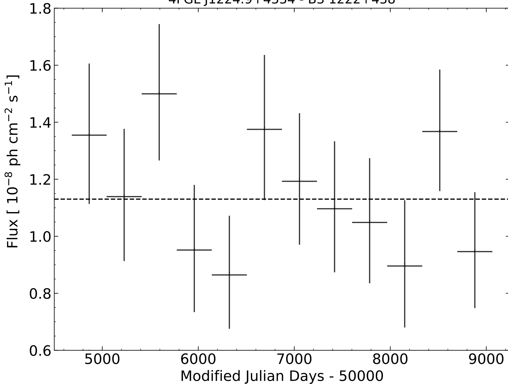
4FGL J1224.9+4334 - B3 1222+438
