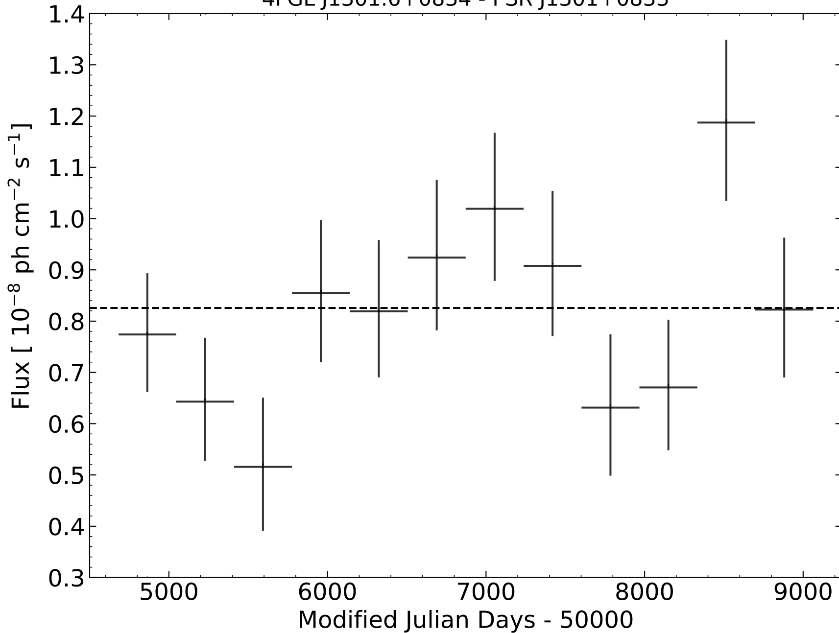
4FGL J1301.6+0834 - PSR J1301+0833
