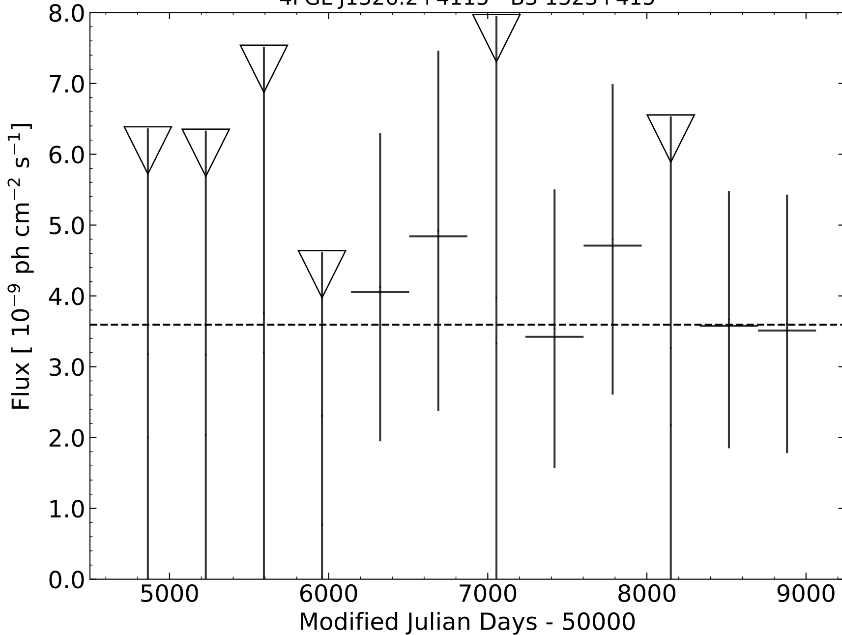
4FGL J1326.2+4115 - B3 1323+415
