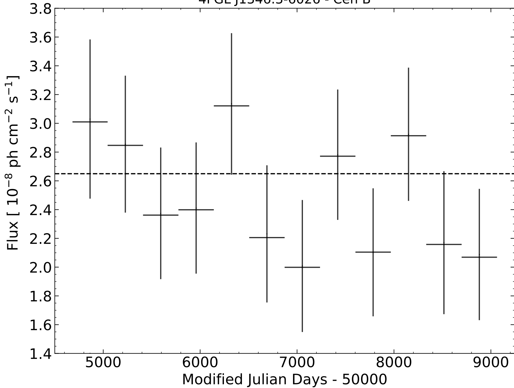
4FGL J1346.3-6026 - Cen B
