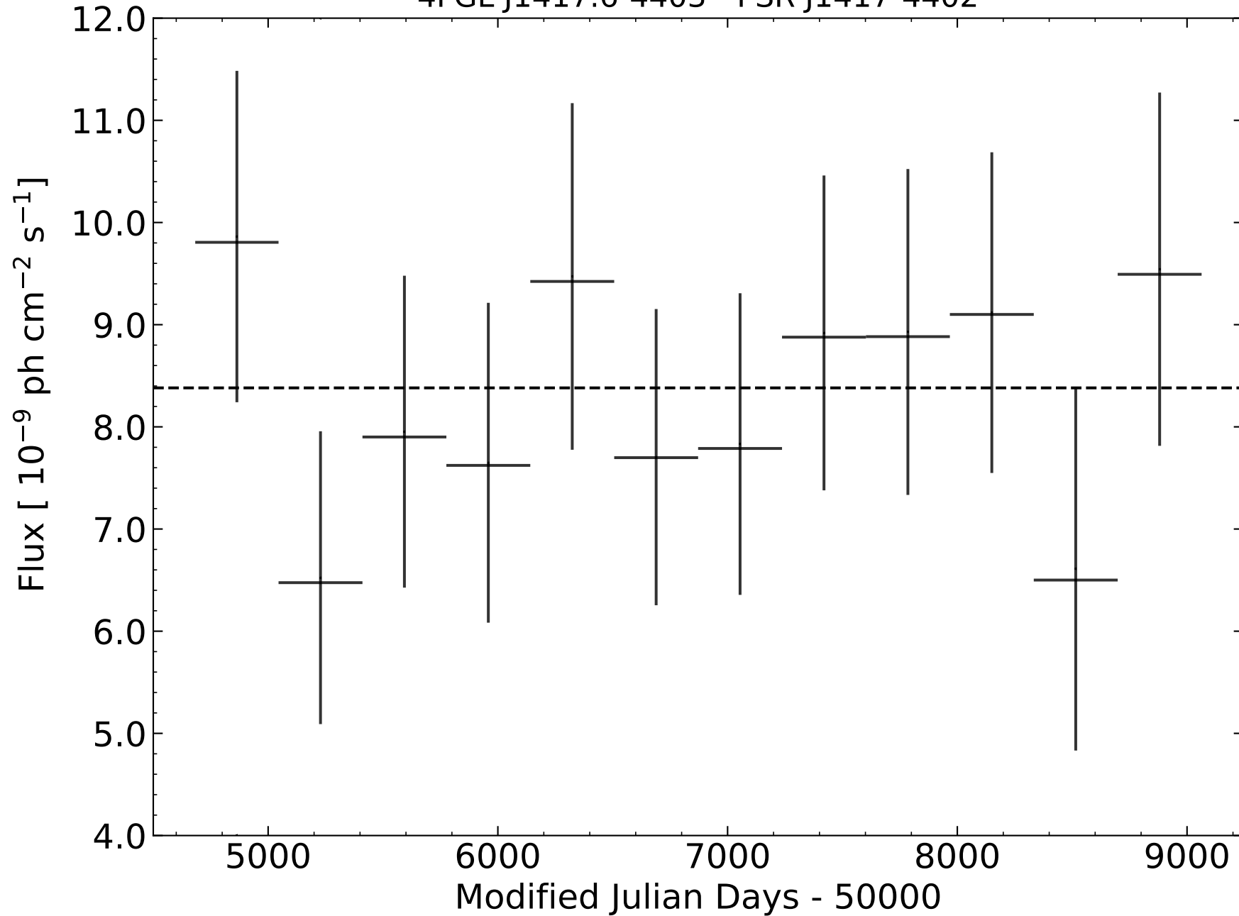
4FGL J1417.6-4403 - PSR J1417-4402
