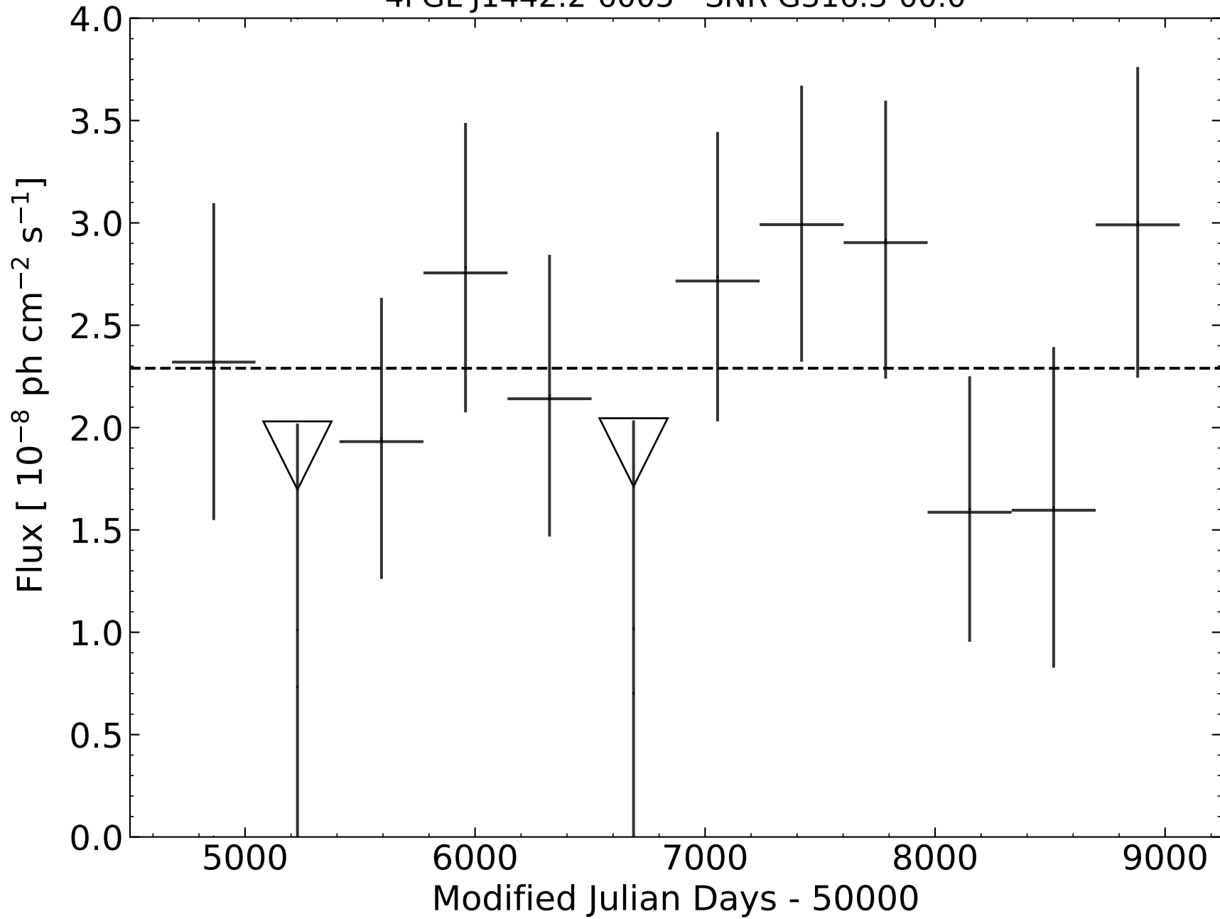
4FGL J1442.2-6005 - SNR G316.3-00.0
