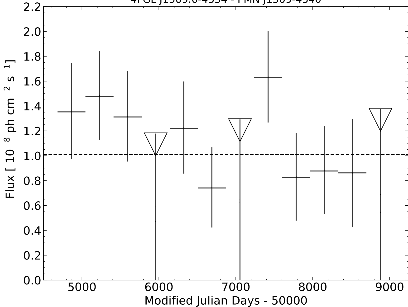
4FGL J1509.6-4334 - PMN J1509-4340
