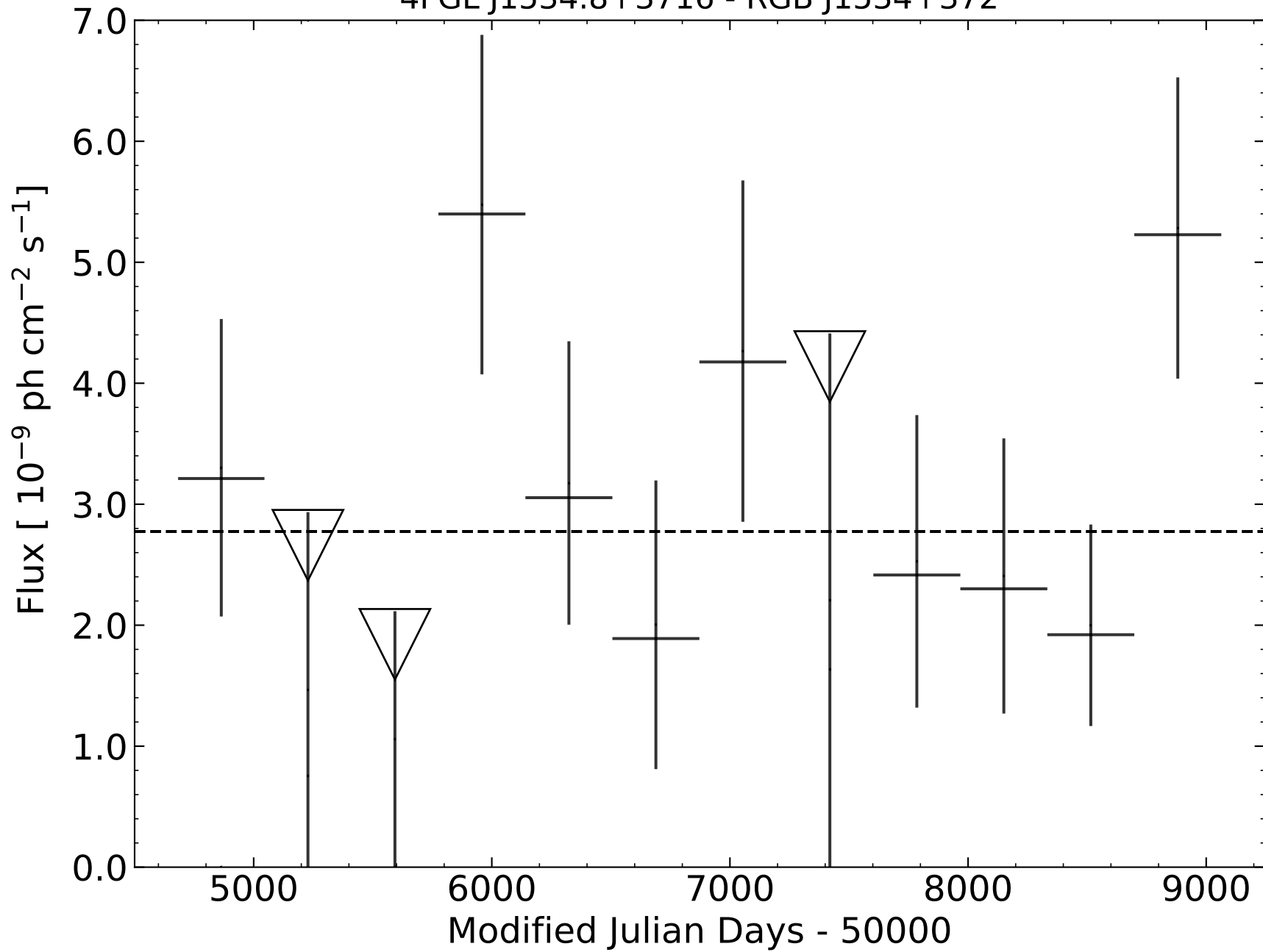
4FGL J1534.8+3716 - RGB J1534+372
