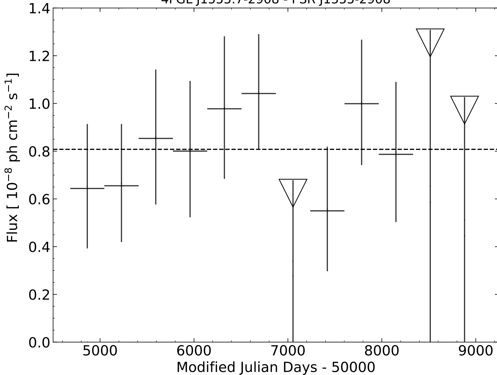
4FGL J1555.7-2908 - PSR J1555-2908
