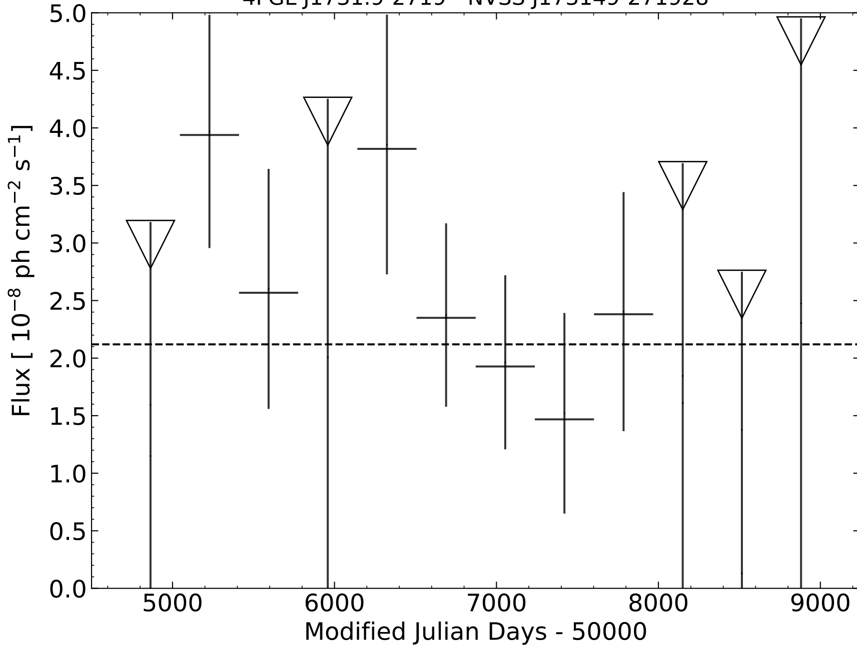
4FGL J1731.9-2719 - NVSS J173149-271928
